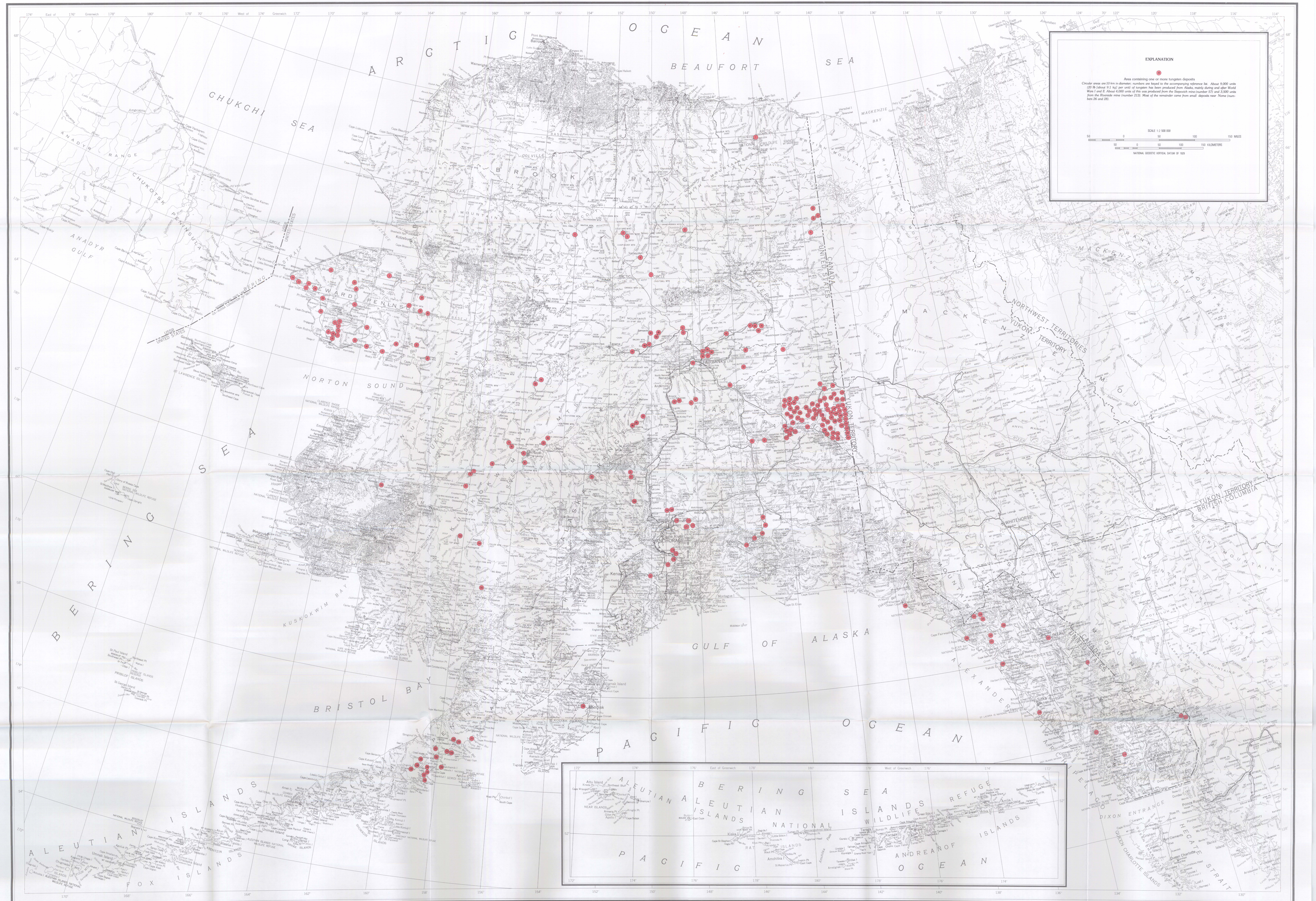
MAP SHOWING OCCURRENCES OF TUNGSTEN MINERALS IN ALASKA
