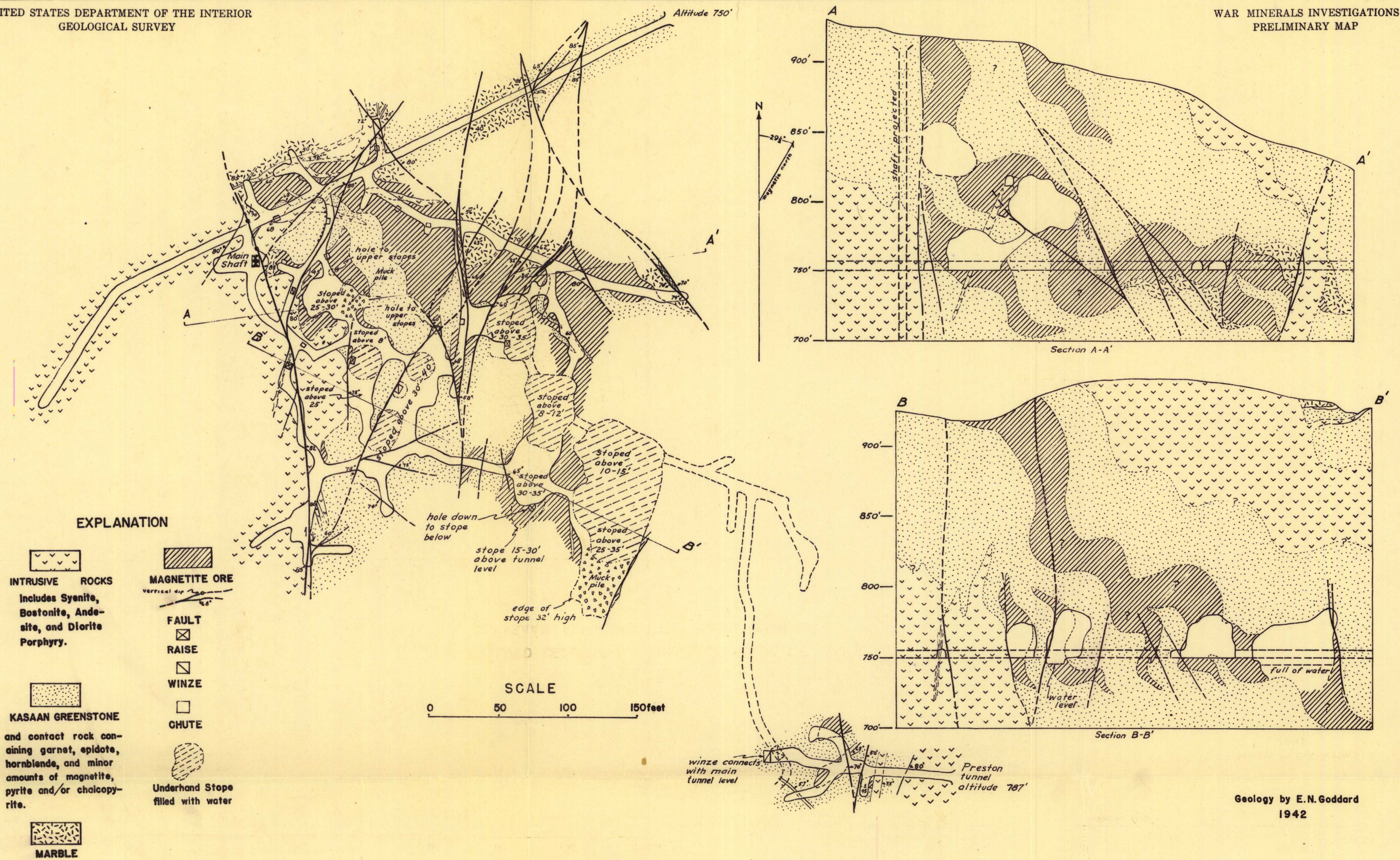
FIGURE 5 GENERALIZED GEOLOGIC MAP AND SECTIONS OF THE MAMIE MINE KASAAN PENINSULA, SOUTHEASTERN ALASKA.
