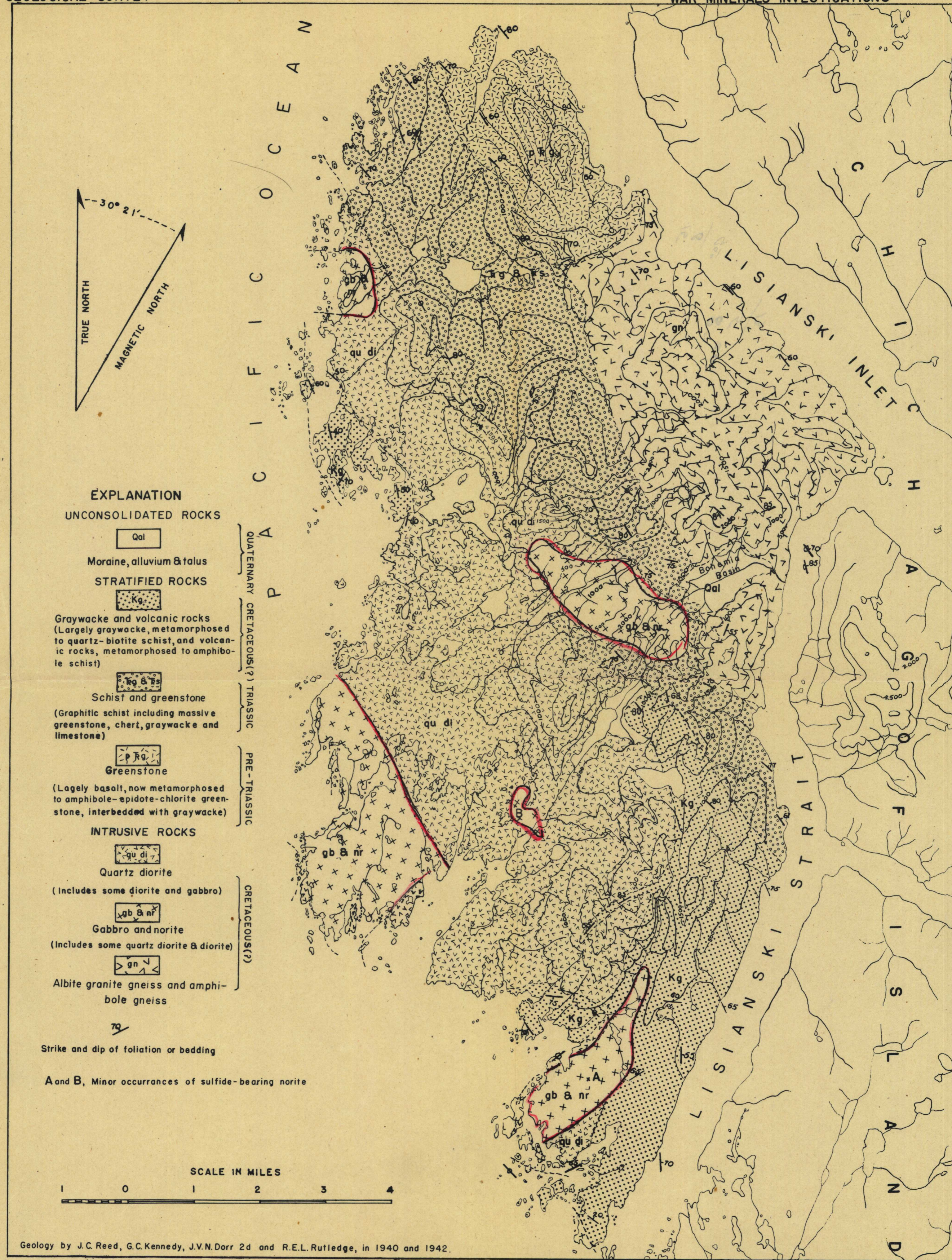
FIGURE 2. - GEOLOGIC MAP OF YAKOBI ISLAND, SOUTHEASTERN ALASKA
