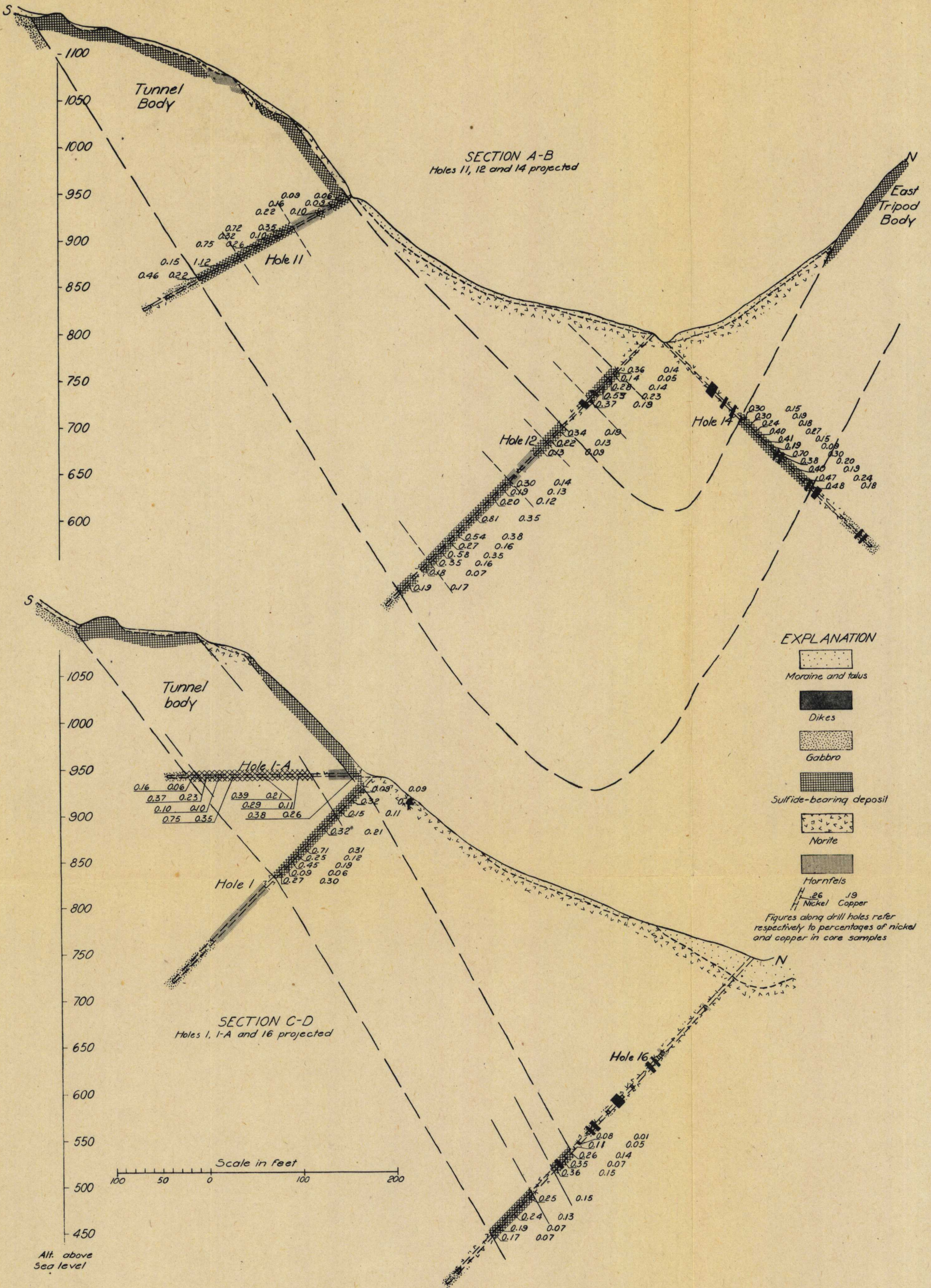
Fig. 5 Geologic sections across sulfide-bearing deposit, Yakobi Island, Alaska (For locations of sections see fig. 3)
