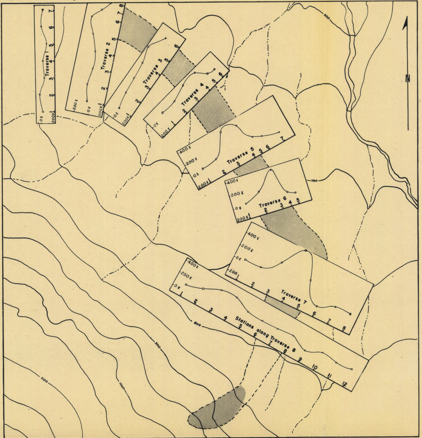
FIG. 7. - MAP, WITH SECTIONS SHOWING MAGNETIC ANOMOLIES ALONG TRAVERSES ACROSS THE MUSKEG DEPOSIT, BOHEMIA BASIN, YAKOBI ISLAND, ALASKA
