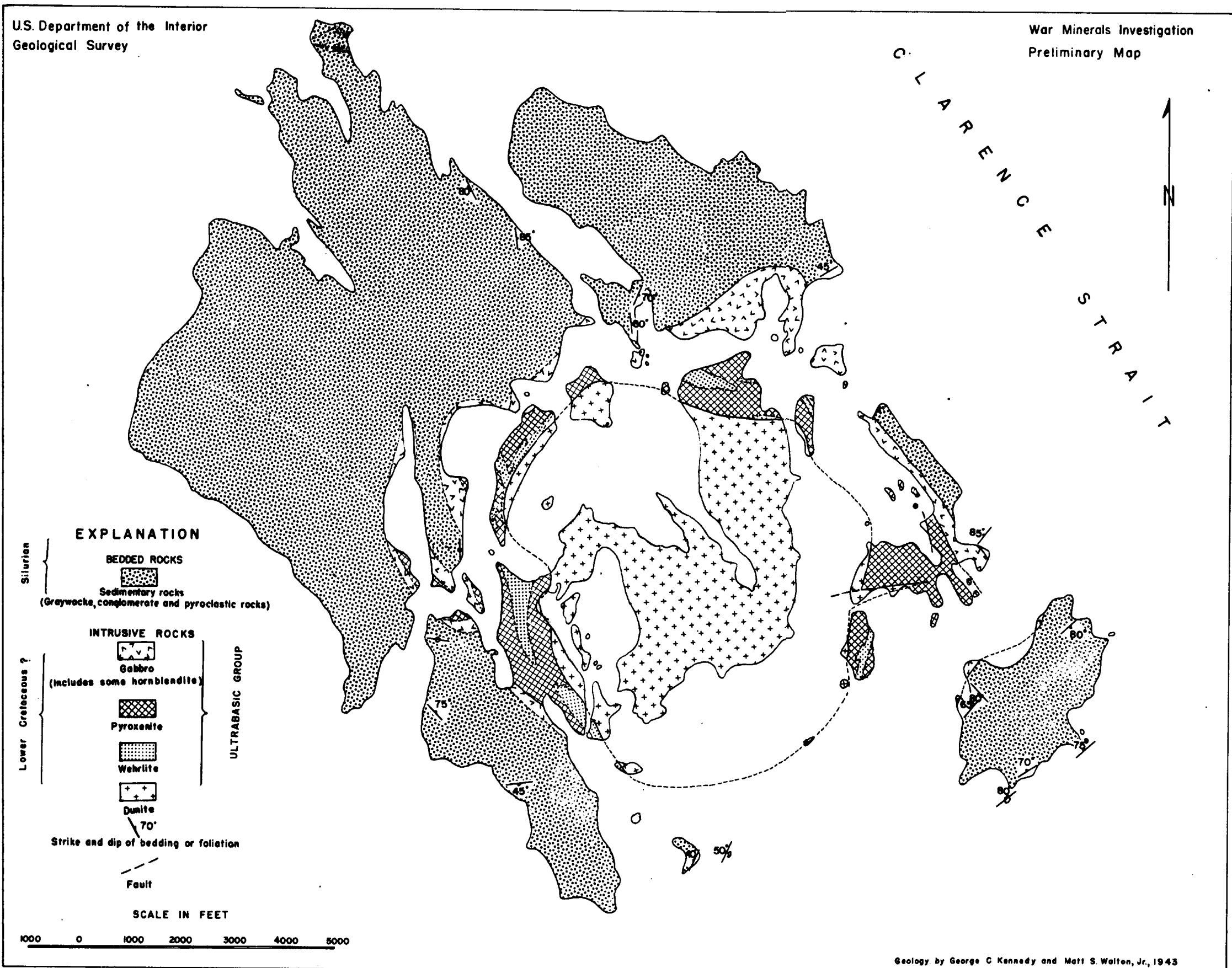
FIGURE 2. — GENERALIZED GEOLOGIC MAP OF THE BLASHKE ISLANDS, SOUTHEASTERN ALASKA
