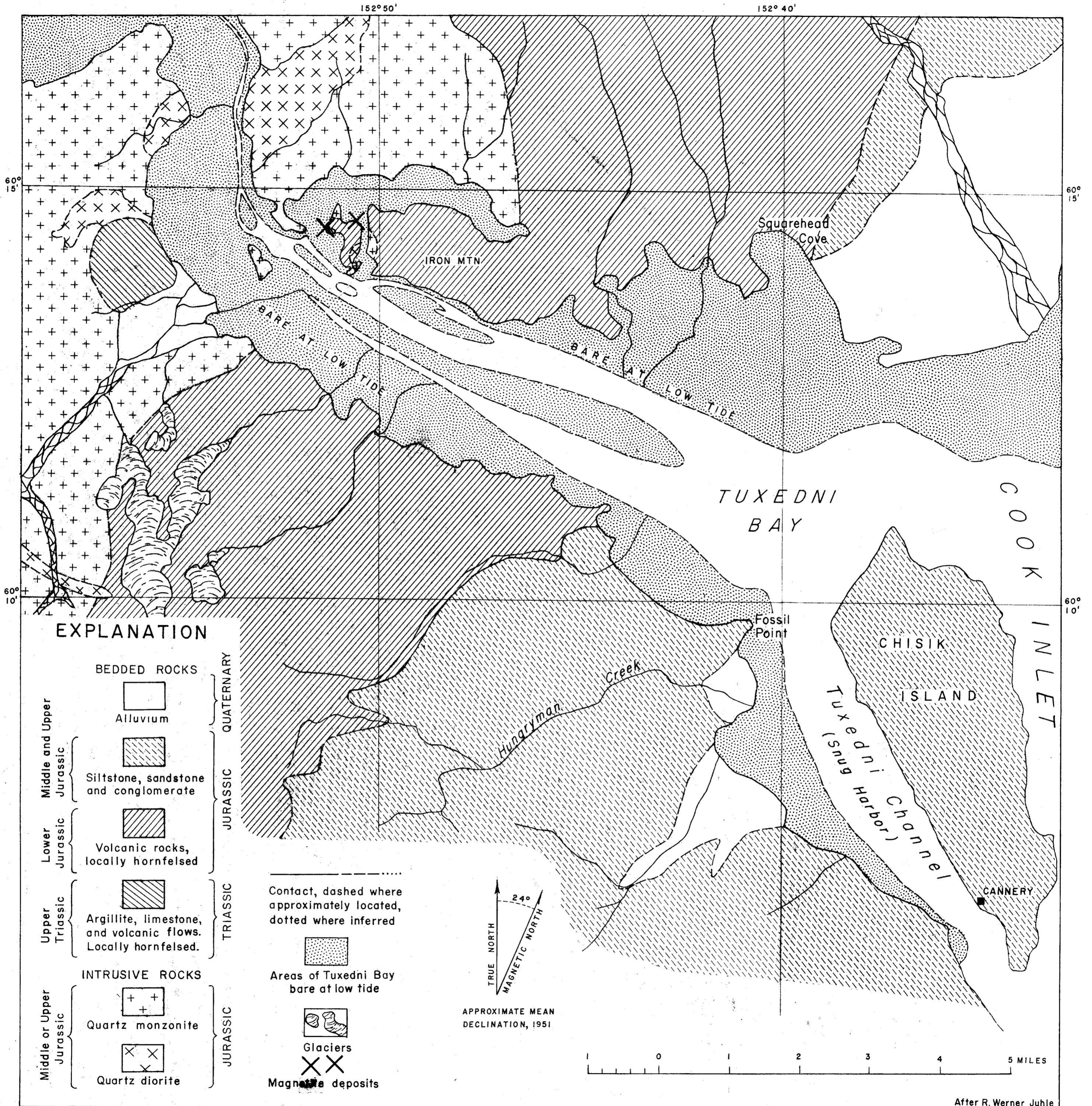
GEOLOGIC MAP OF THE TUXEDNI BAY AREA SHOWING THE LOCATION OF MAGNETITE DEPOSITS
