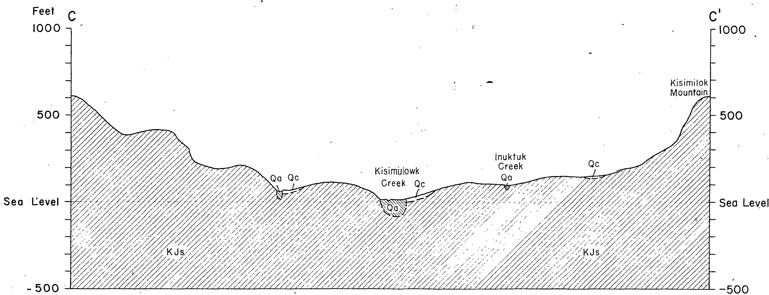
Cross-section through Site 2
