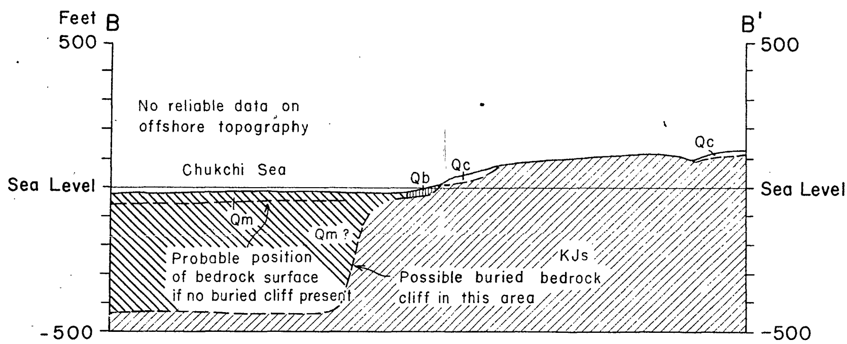
Cross-section through Site 1 showing alternate interpretations of offshore geology
