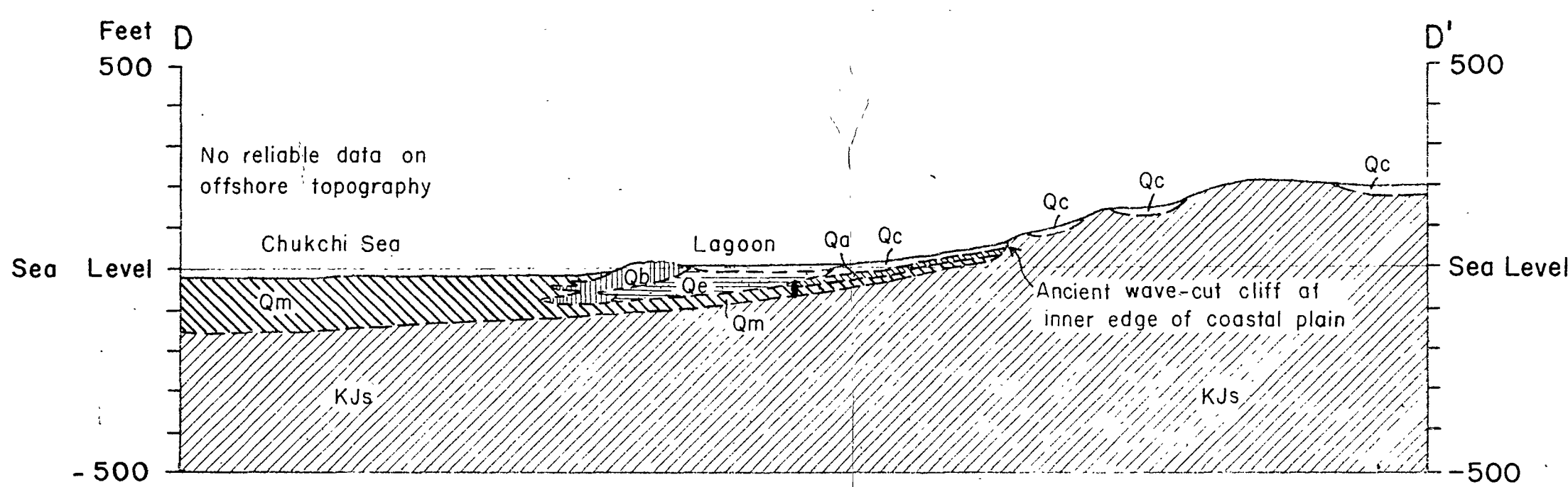
Cross-section through Site 3
