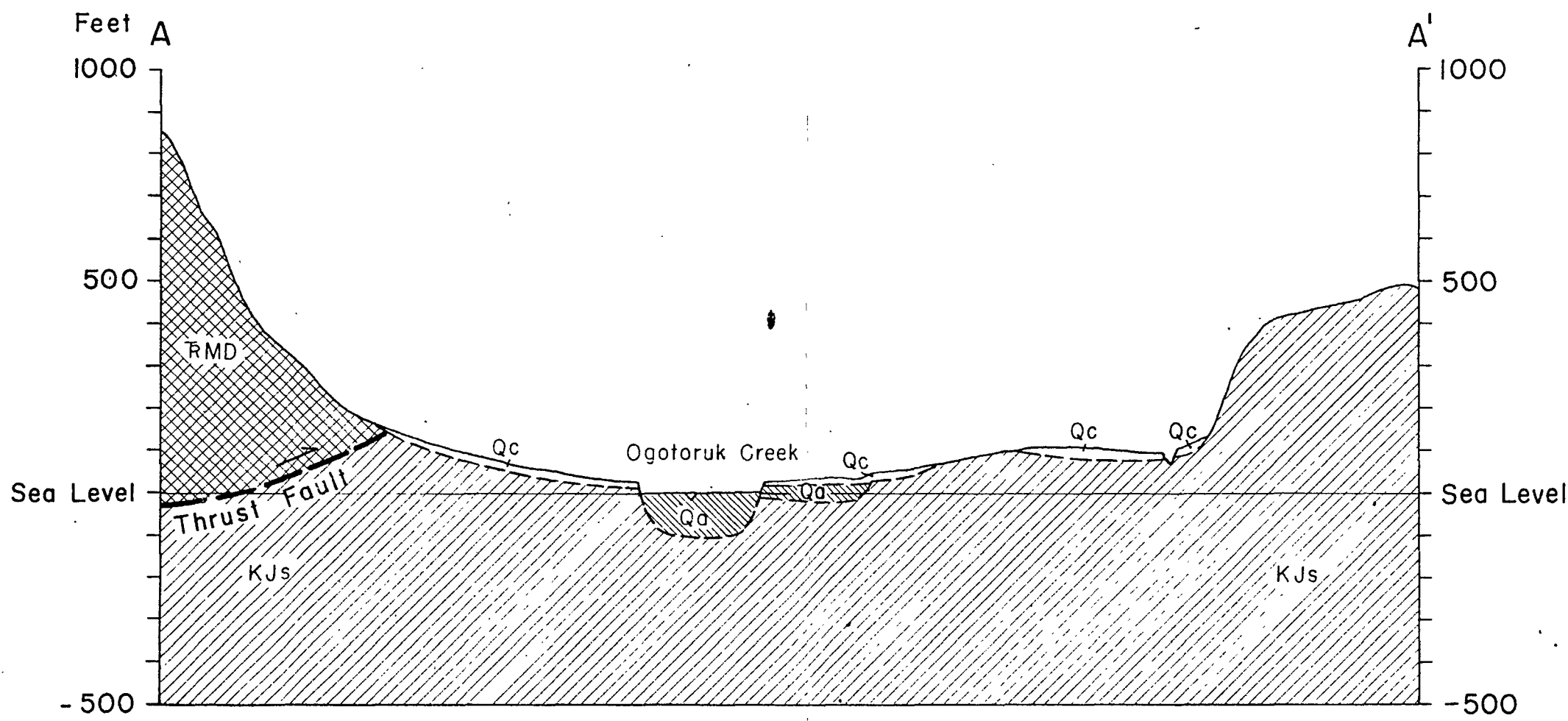
Cross-section through Site 1
