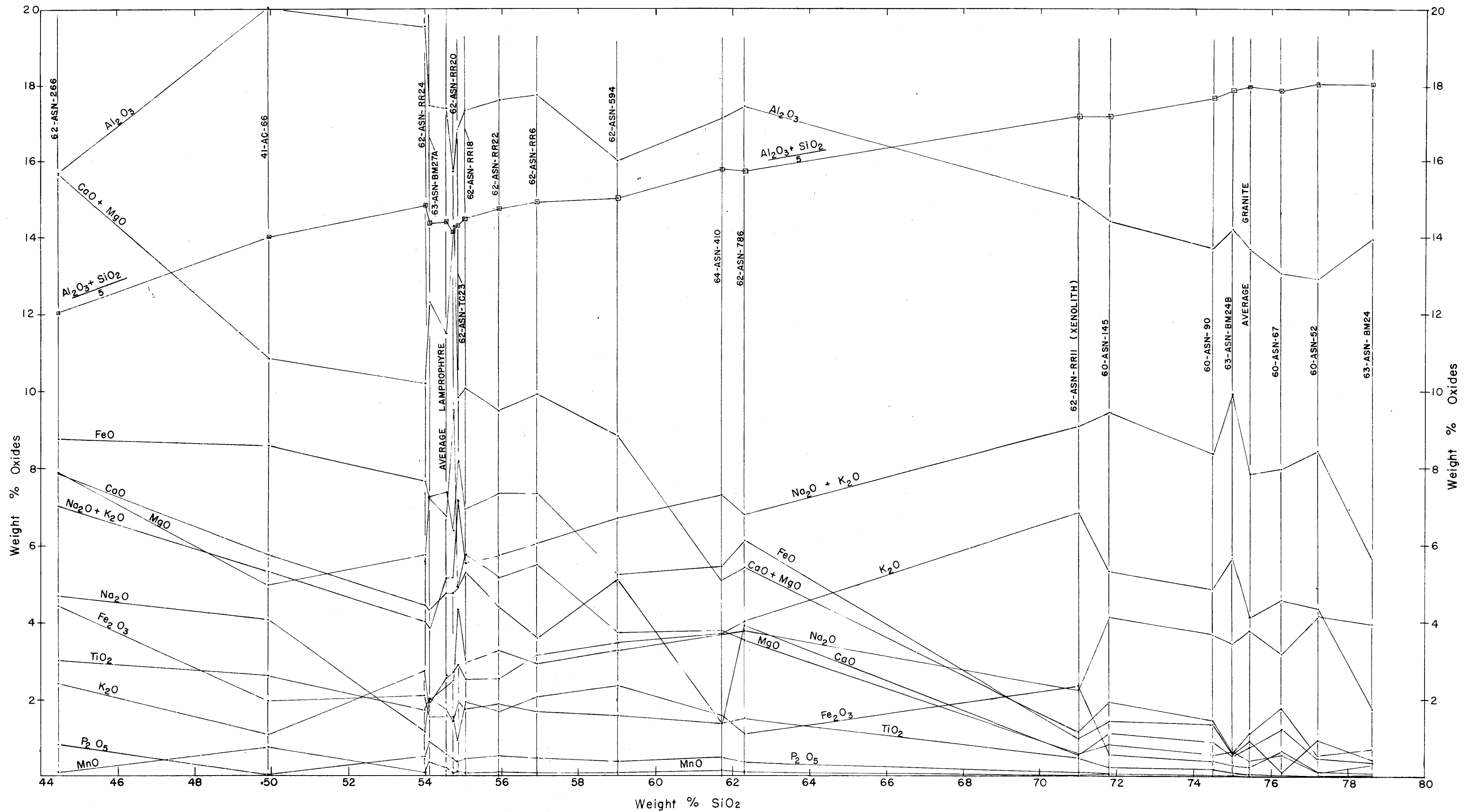
FIGURE 22 LARSEN DIAGRAM SHOWING VARIATION IN OXIDES IN IGNEOUS ROCKS OF THE YORK MOUNTAINS, WESTERN SEWARD PENINSULA, ALASKA
