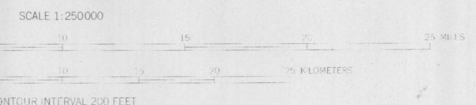
METALLIC MINERAL RESOURCES MAP OF THE ANCHORAGE QUADRANGLE, ALASKA Compiled by Edward H. Cobb and Neal A. Matson, Jr. 1969
