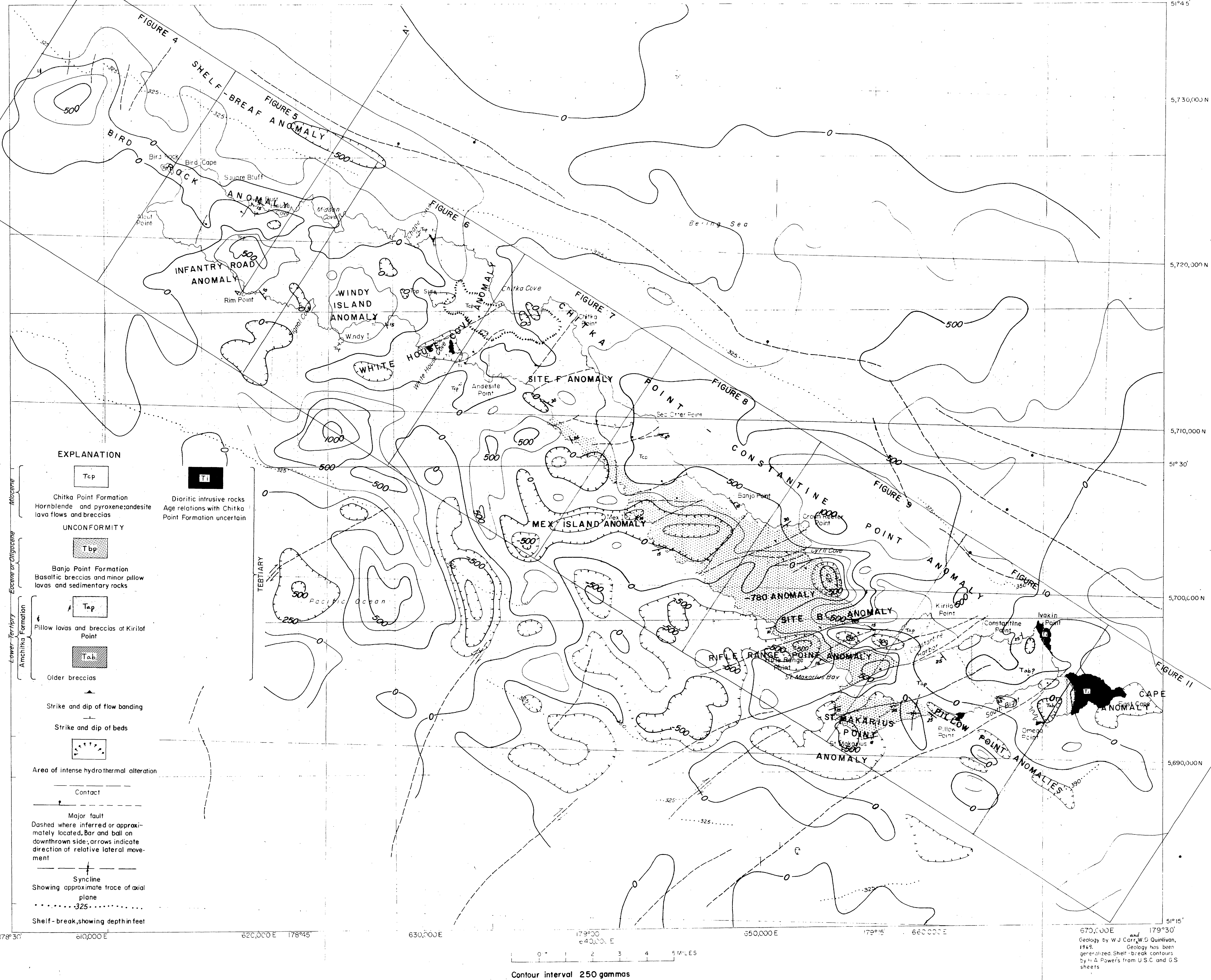
FIGURE 3.--RESIDUAL MAGNETIC ANOMALY AND GENERALIZED GEOLOGIC MAP OF AMCHITKA ISLAND, ALASKA. INSERTS SHOW OUTLINES OF FIGURES 4 THROUGH 11 WHICH SHOW IN GREATER DETAIL THE RESIDUAL ANOMALIES. LABELED ANOMALIES ARE DISCUSSED IN THE TEXT.
