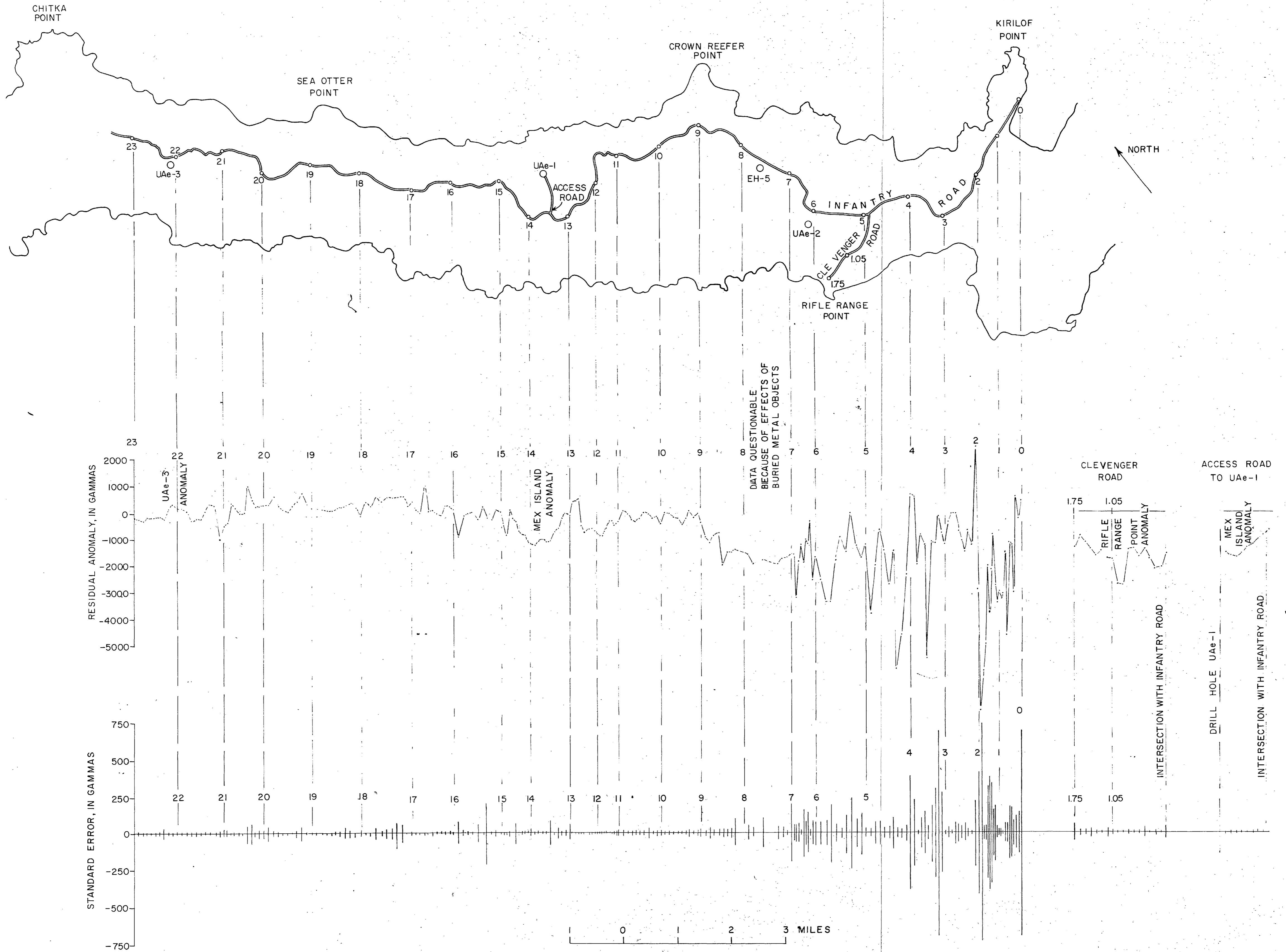
FIGURE 12.--PLOTS OF MAGNETIC ANOMALY AND STANDARD ERROR FROM GROUND SURVEY DATA AT STATIONS 0.1 MILE APART ALONG THE INFANTRY ROAD FROM MILE 0 ON KIRILOF POINT TO MILE 23 NORTHWEST OF DRILL HOLE Uae-3, ALONG CLEVENGER ROAD, AND ALONG THE ACCESS ROAD TO DRILL HOLE Uae-1. AT EACH STATION, THE DATA FROM FIVE OBSERVATIONS SPACED 5 FEET APART ARE AVERAGED TO GIVE THE MAGNETIC ANOMALY, AND COMPUTED TO GIVE THE STANDARD ERROR.
