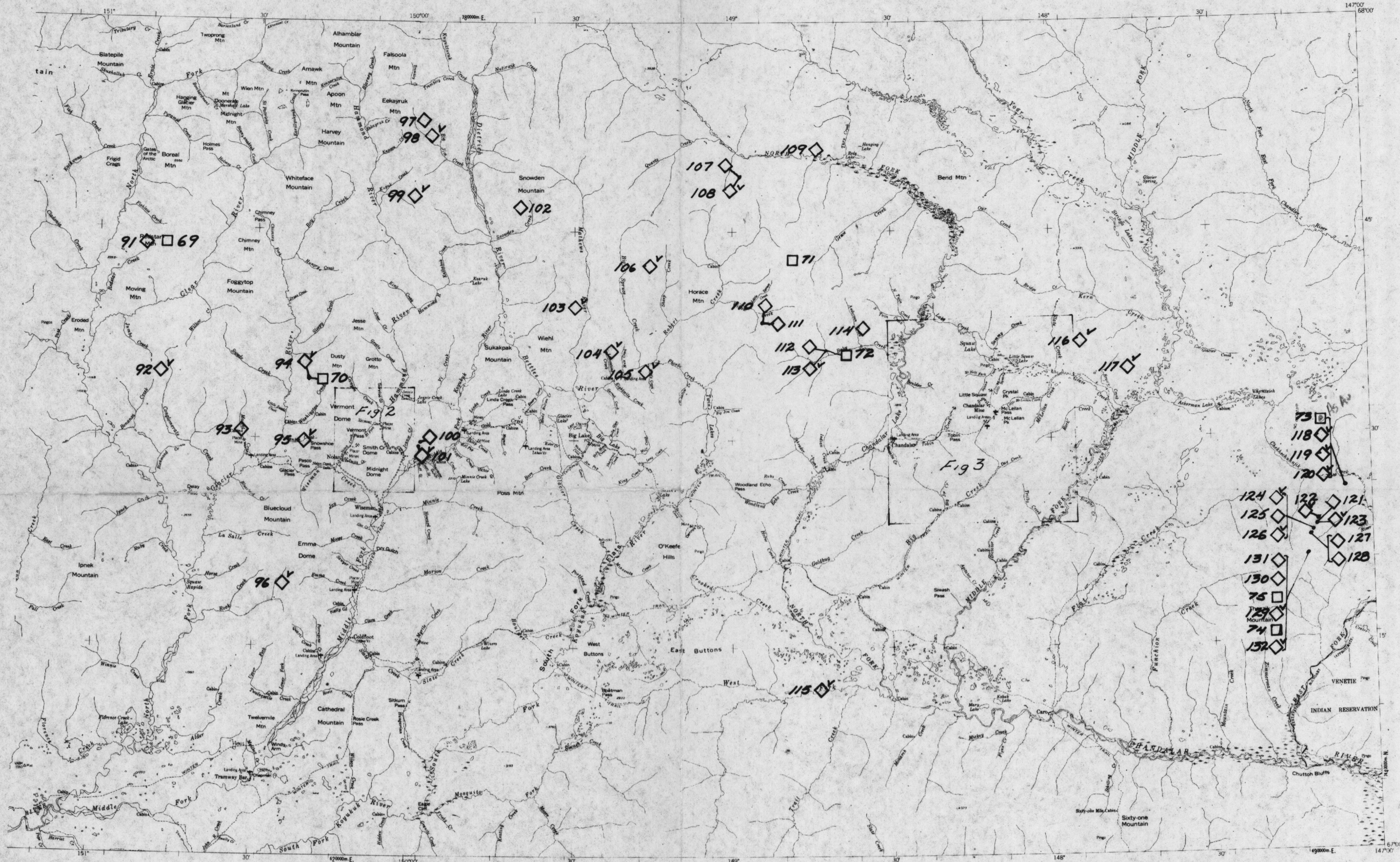
Fig 1 Rock and soil sample localities in Chandalar and eastern Wiseman quadrangles See figs 2 and 3 for localities near Wiseman and Chandalar
