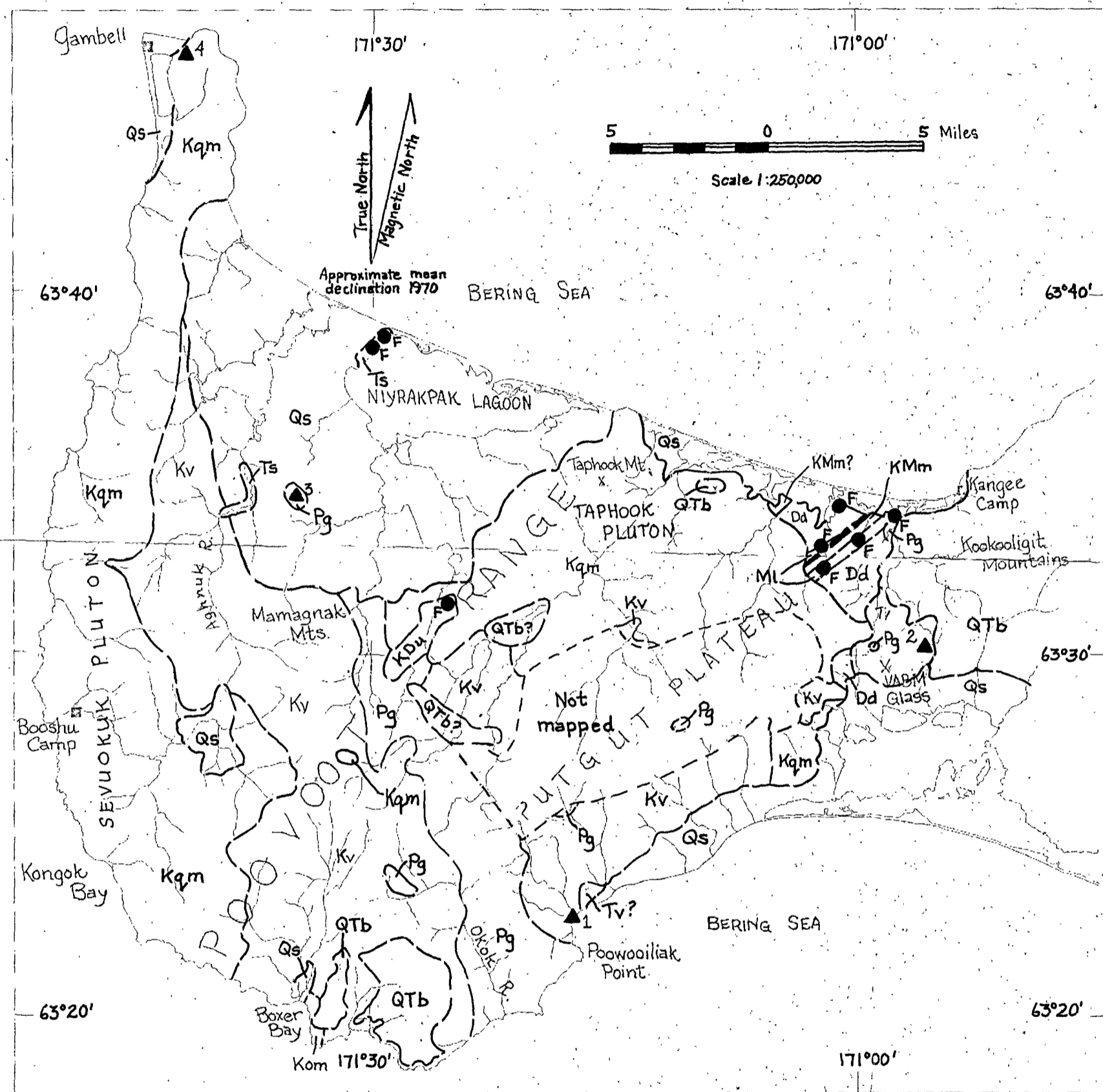
Figure 2. Reconnaissance geologic map of western St. Lawrence Island.
