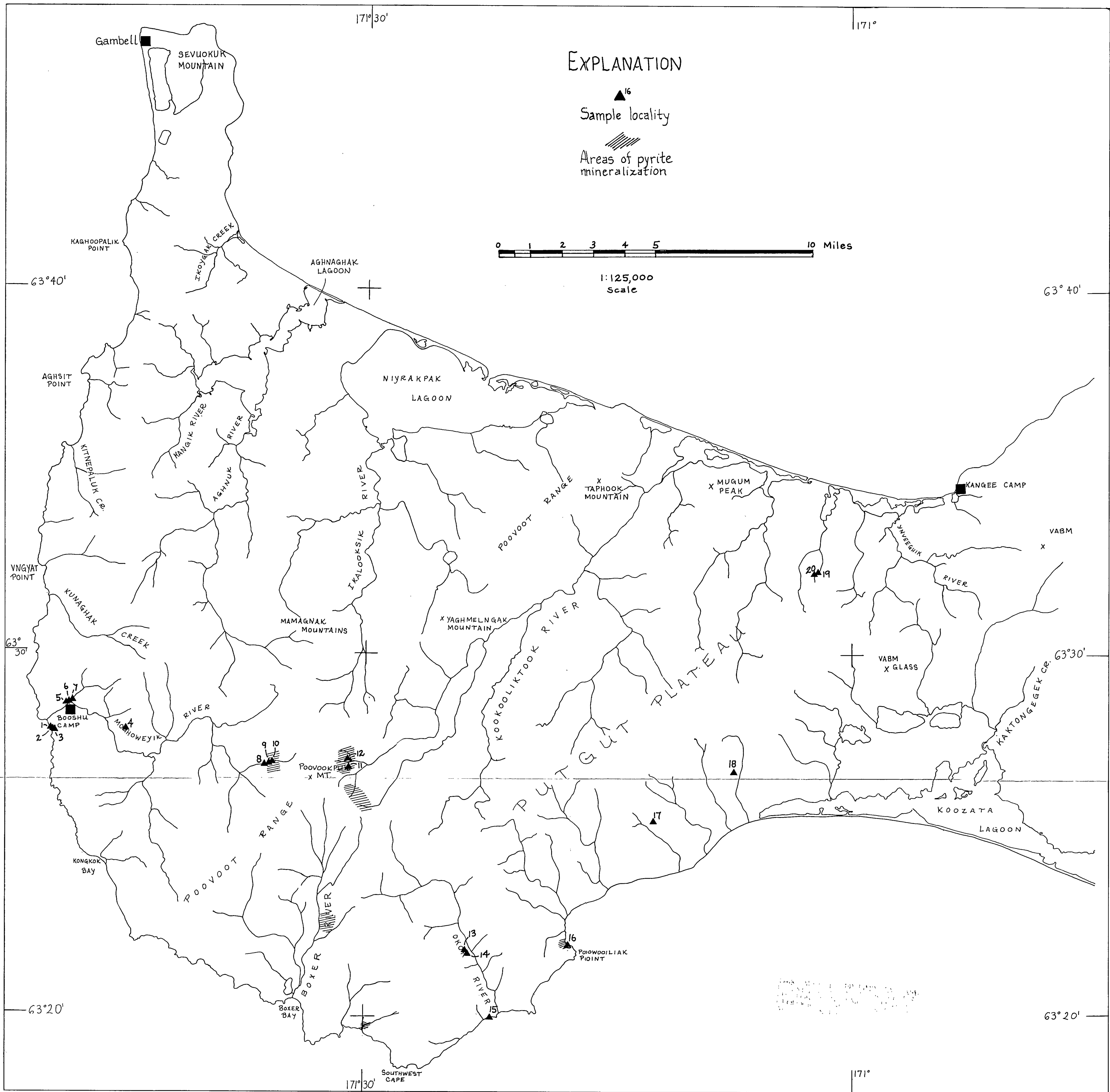
Figure 4. Location of analyzed bedrock samples listed in Table 5.
