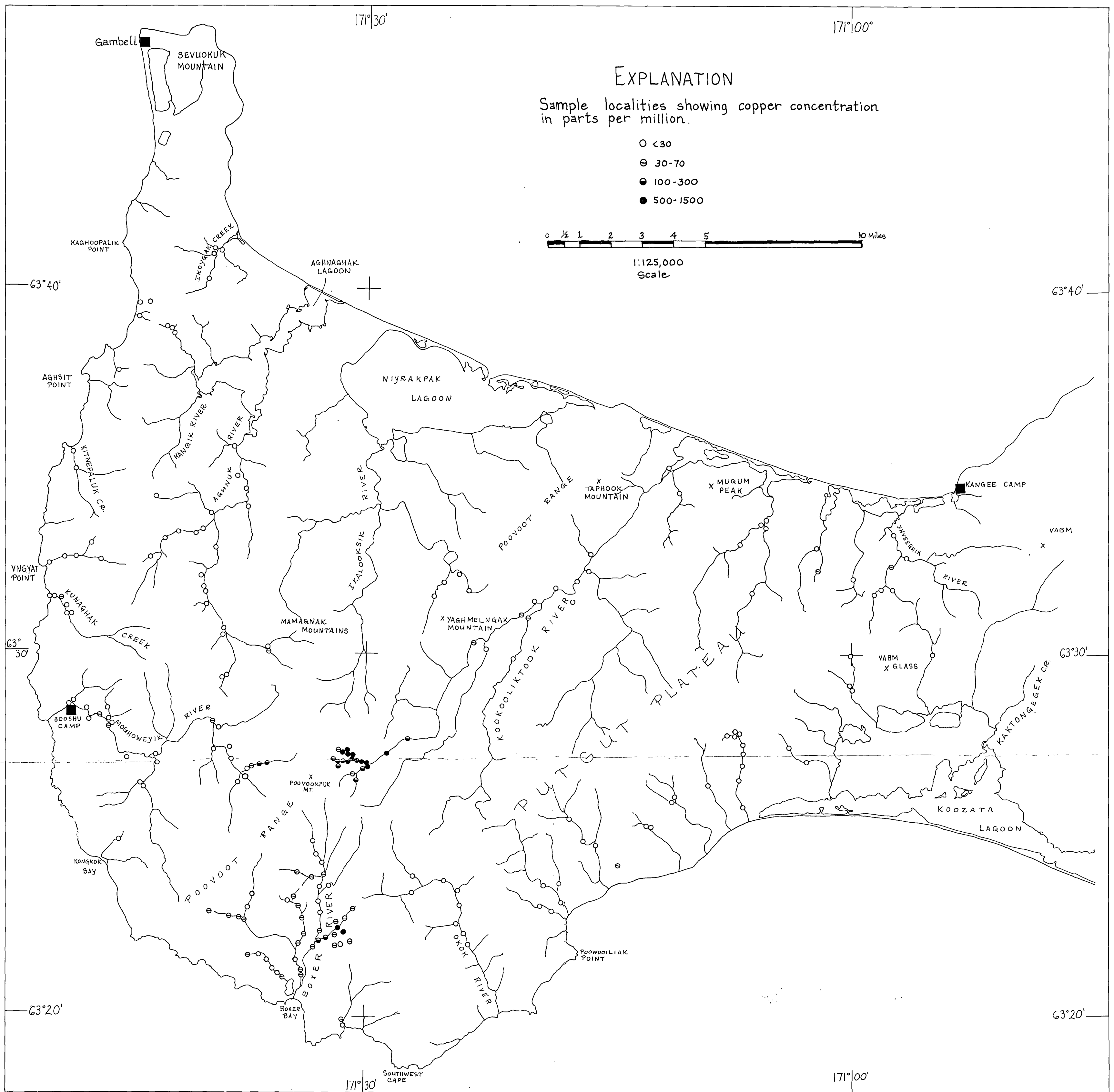
Figure 6. Copper distribution in stream sediment samples of western St. Lawrence Island.
