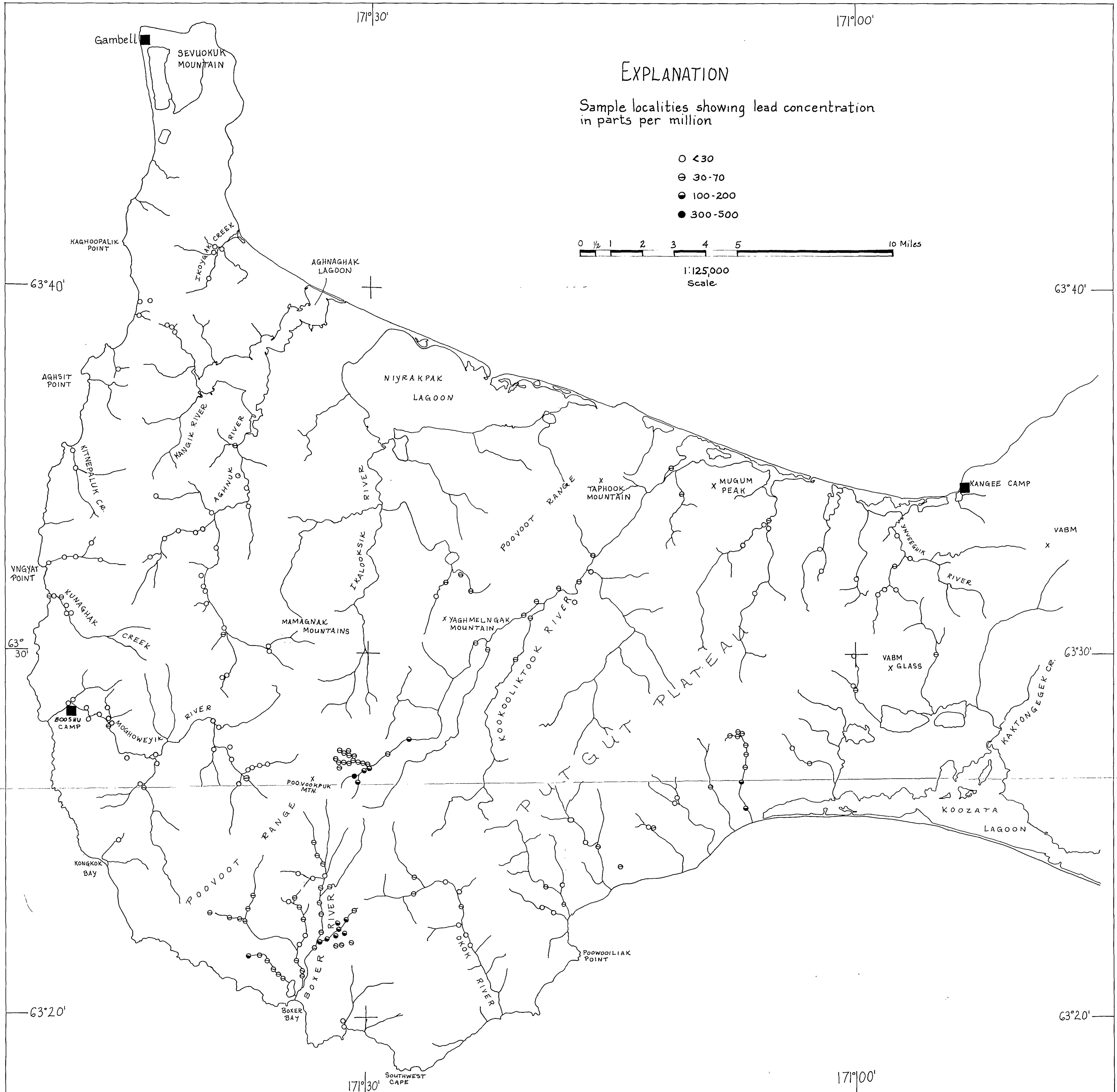
Figure 7. Lead distribution in stream sediment samples of western St. Lawrence Island.
