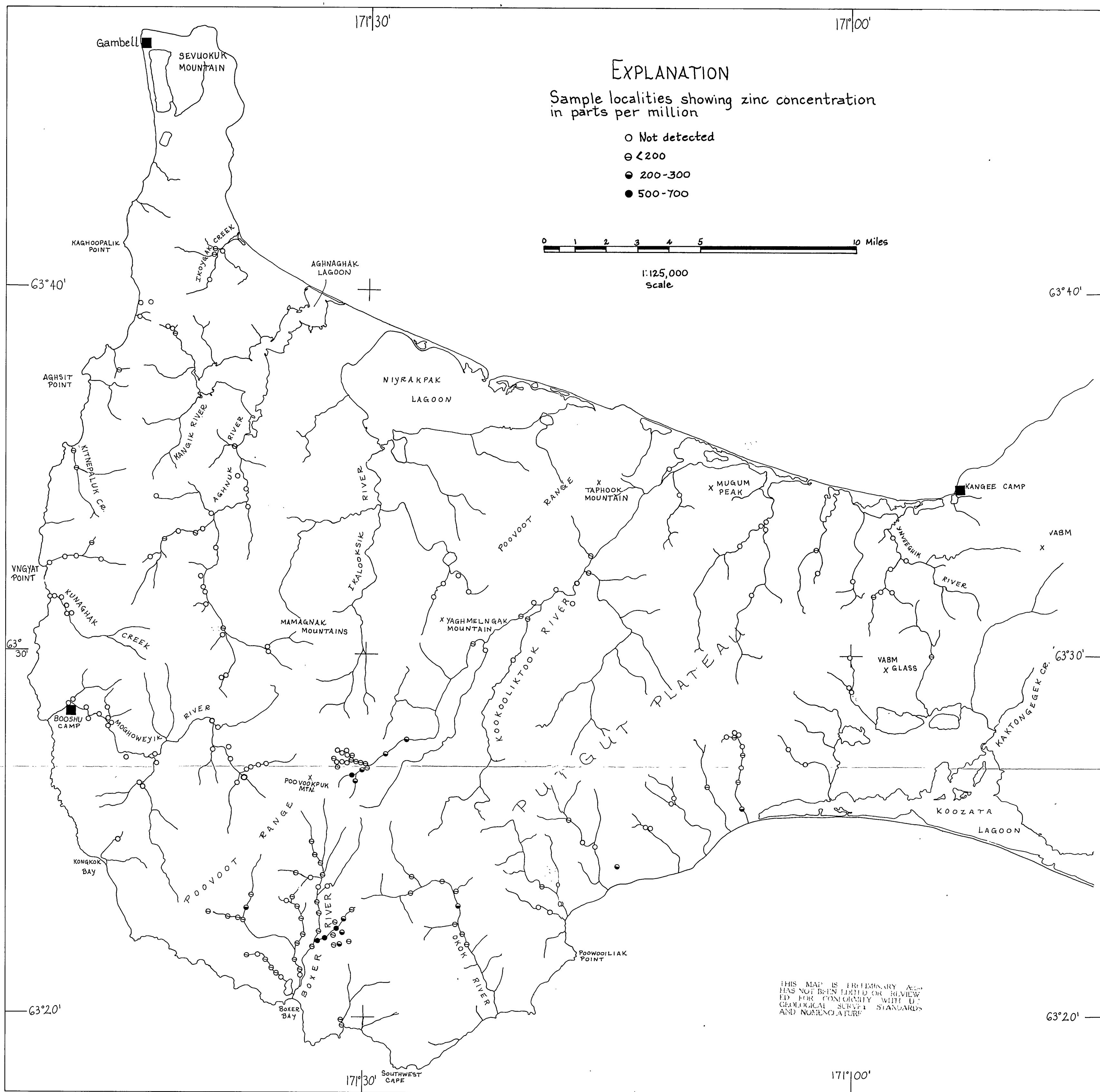
Figure 8. Zinc distribution in stream sediment samples of western St. Lawrence Island.
