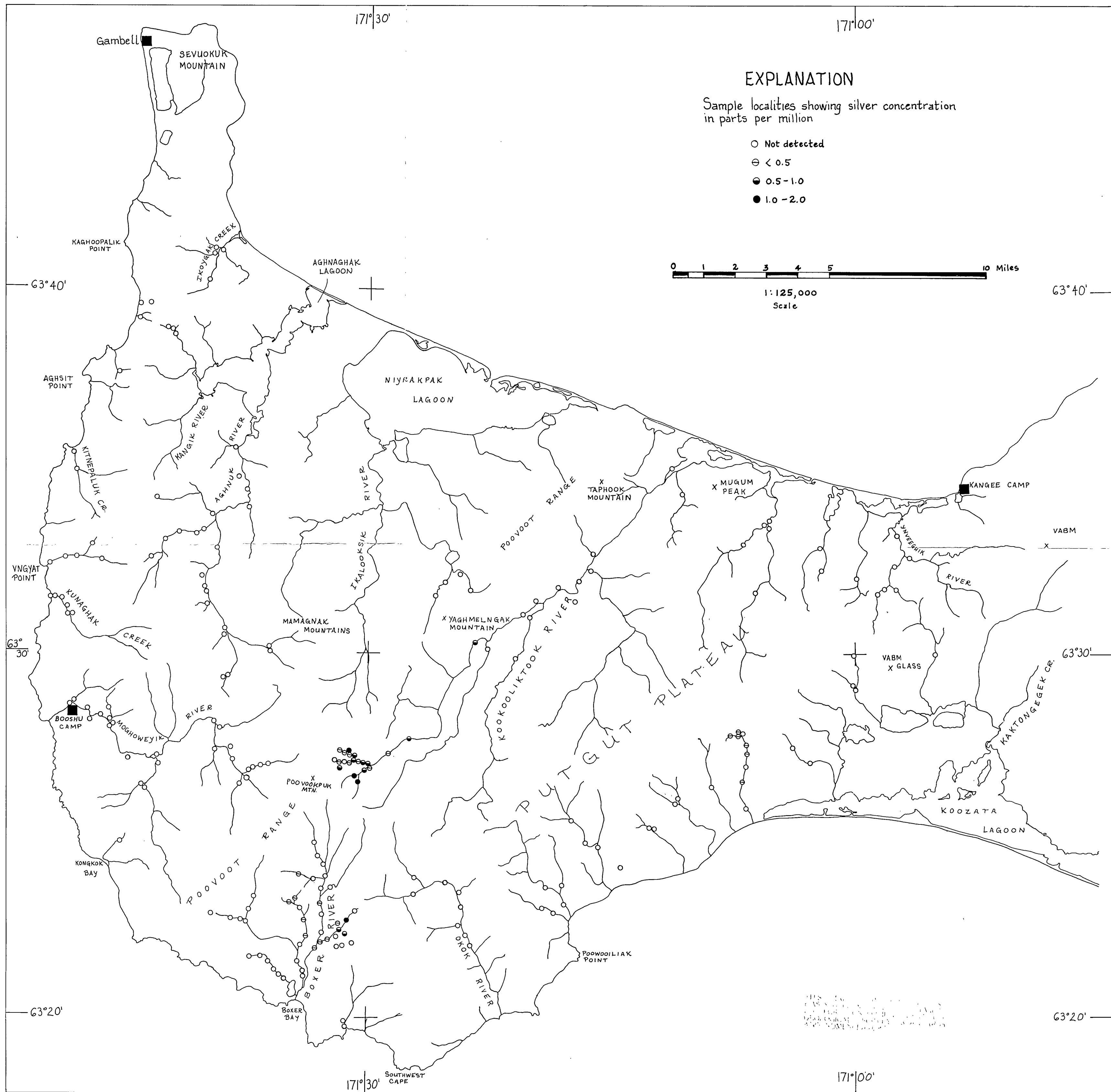
Figure 9. Silver distribution in stream sediments of western St. Lawrence Island.
