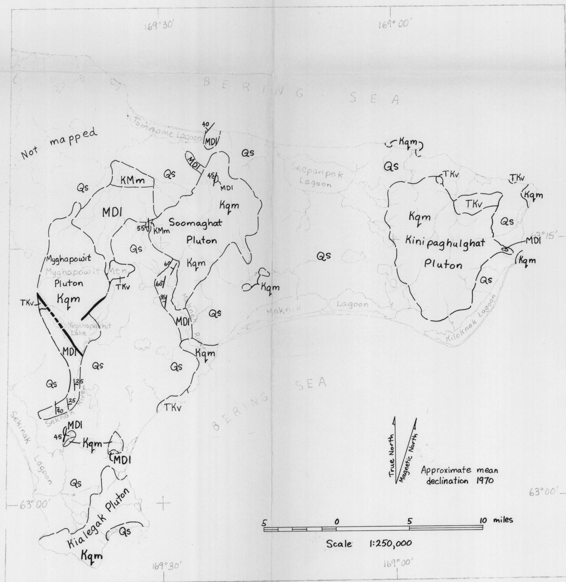
Figure 2. Reconnaissance Geologic map of eastern St. Lawrence Island.
