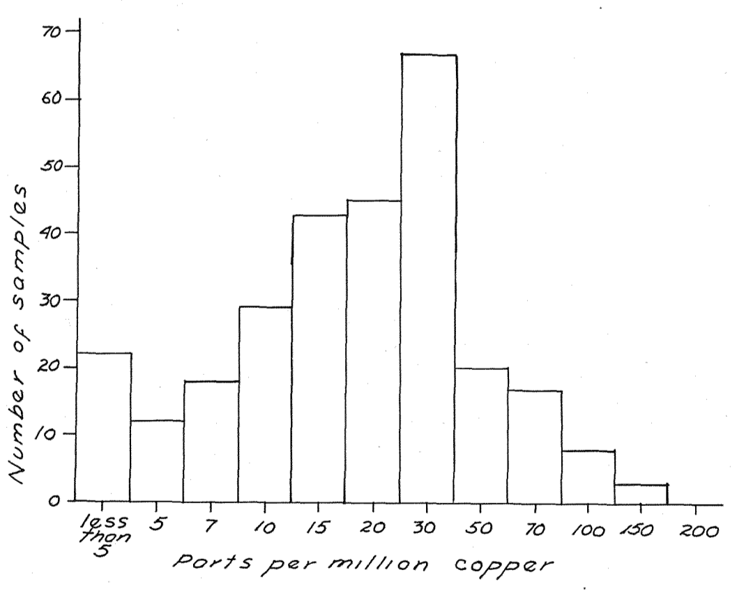
Histograms showing distribution of copper and tin in 284 samples of stream sediments as determined by Spectroscopic method.
