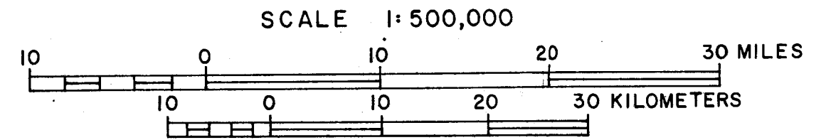
Figure 10 SUMMARY MAP OF METALLIC MINERAL OCCURRENCES, GEOLOGICALLY FAVORABLE AREAS, AND SELECTED GEOCHEMICAL ANOMALIES IN SOUTHERN NPRA
