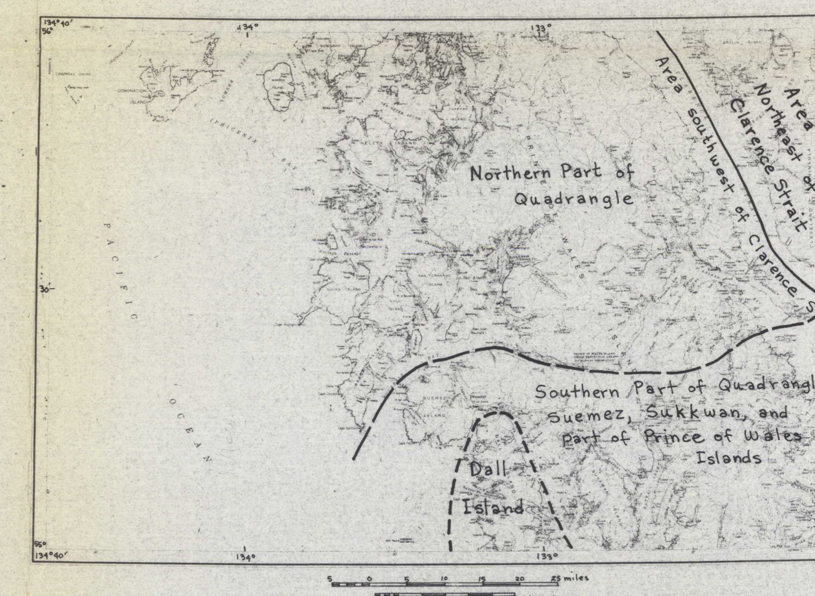
Figure 4. Index map showing geographic limits of regions referred to in the correlation of map units and the description of map units.
