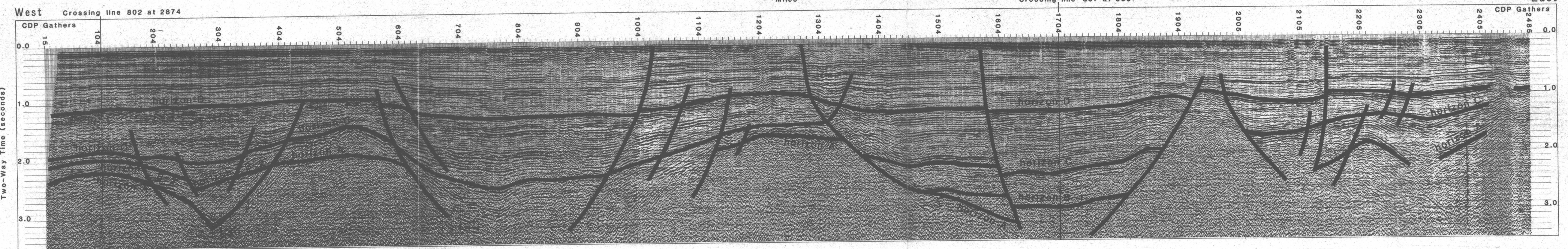
Figure 9. USGS Seismic Line 813.
