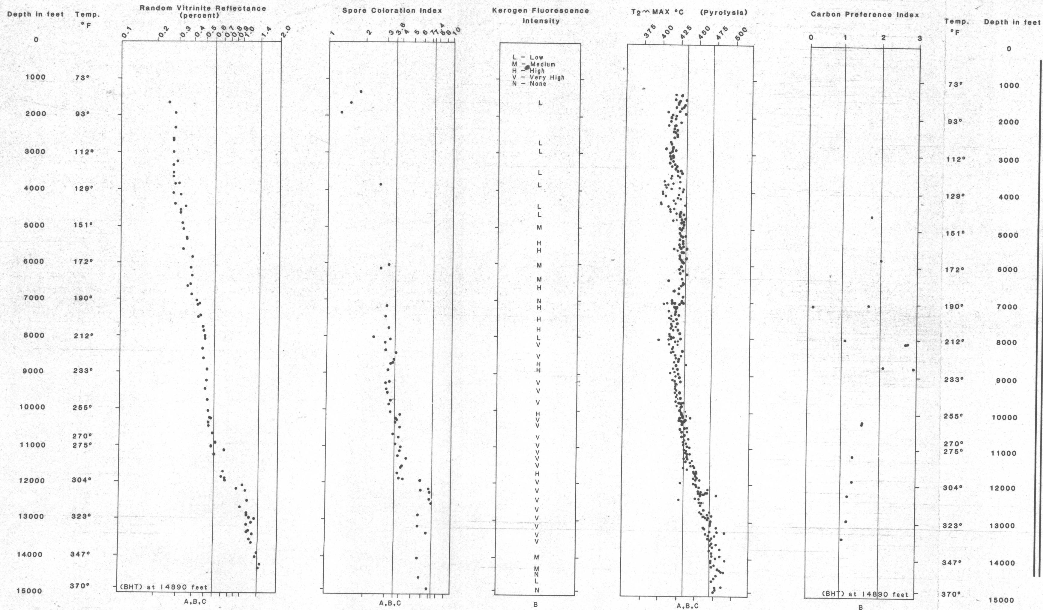
Figure 40. Selected Indicators of Thermal Maturation. [Sample Sources: A-Cuttings, B-Sidewall Cores, C-Conventional Cores]
