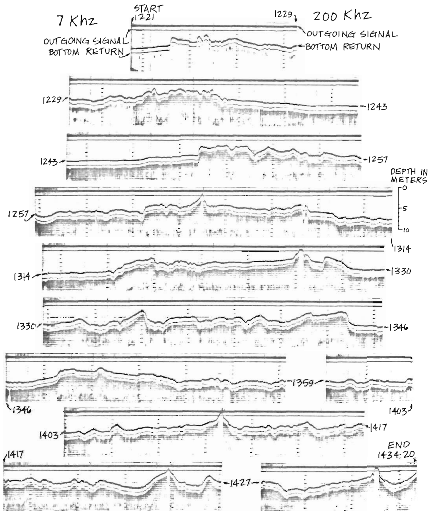
Figure 4. 200 kHz fathometer and 7 kHz sub-bottom profiles recorded along and keyed by time to tracklines of figure 1. (Prepared at Marine Science Data Center, Project Chief T.E. Chase, by Jeff Young).
