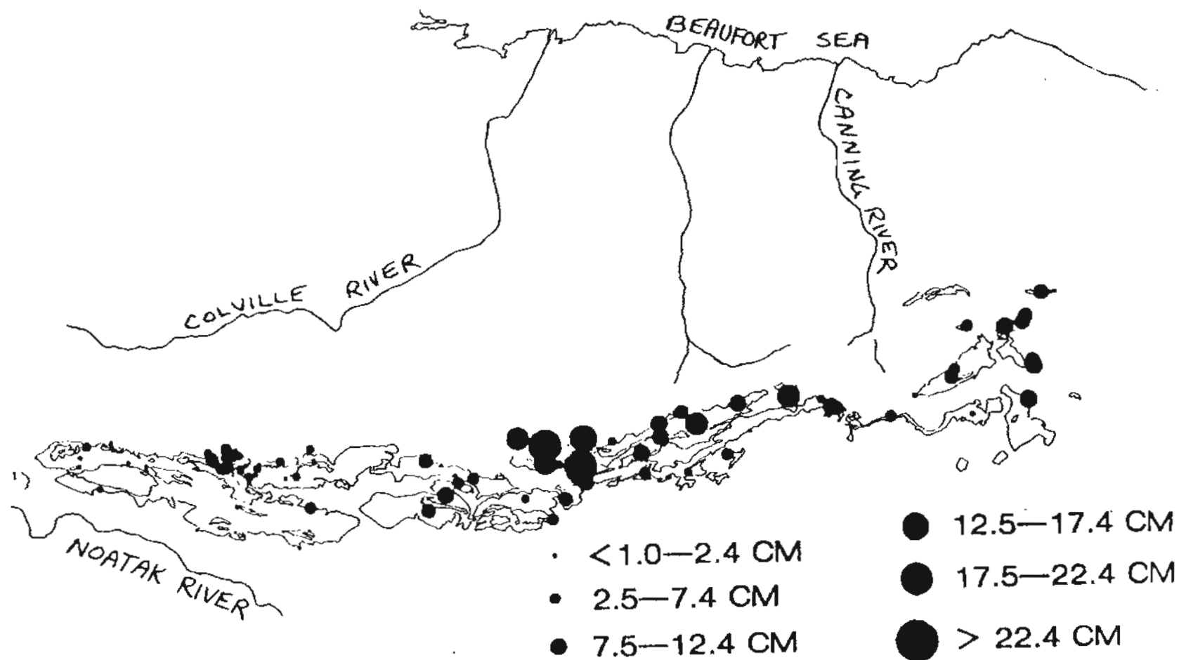
Figure 9.--Map showing distribution of the largest conglomerate clasts in the Kanayut Conglomerate.
