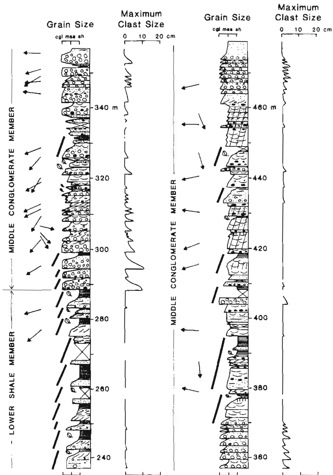
Figure 6A, 6B, 6C.--Measured section of the lower shale member, middle conglomerate member, and Stuver Member of the Kanayut Conglomerate near the Junjik River at station 79 Bl36, eastern Brooks Range. See Figure 3 for location of section.
