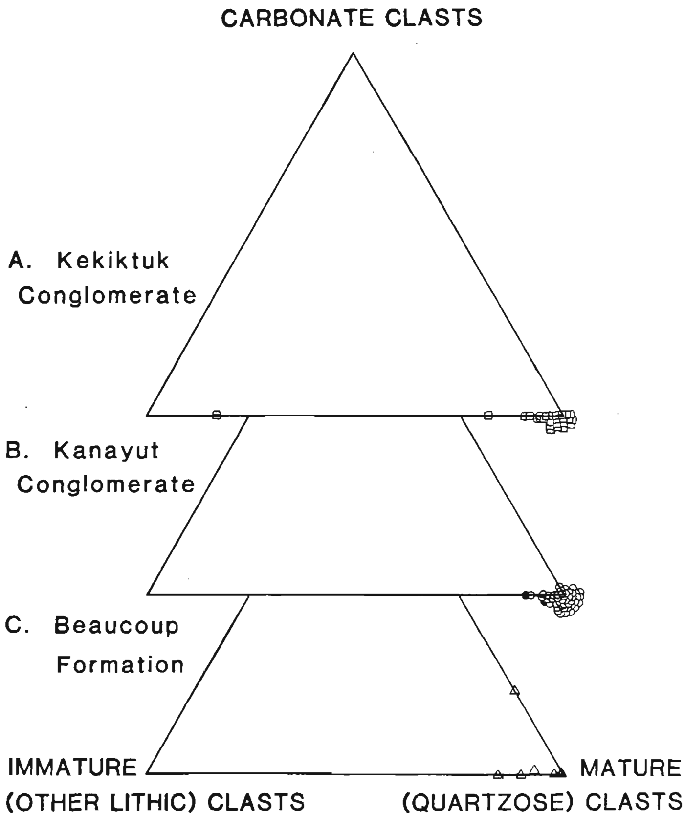
Figure 11.--Immature clast (argillite, siltstone, sandstone and greenstone)--carbonate clast--mature clast (chert, vein quartz, and quartzite) ternary diagram from pebble counts made during the 1978 and 1979 field seasons. A, Kekiktuk Conglomerate. B, Kanayut Conglomerate; filled circles = conglomerate from the Hunt Fork Shale. C, Conglomerate from the Beaucoup Formation.
