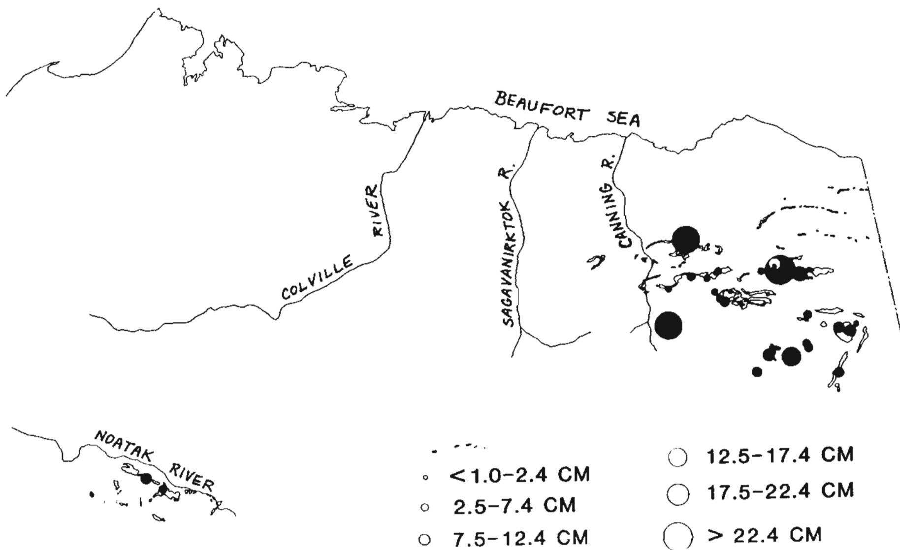
Figure 10.--Map showing distribution of the largest conglomerate clasts in the Kekiktuk Conglomerate.
