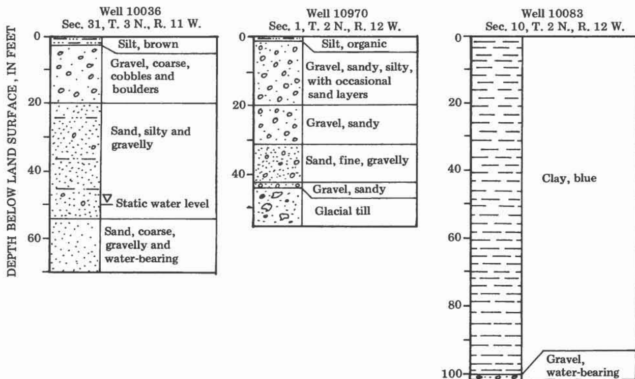
Figure 5.--Logs of selected wells in the Johnson Lake - Crooked Creek area. Locations of wells are shown in figure 4.
