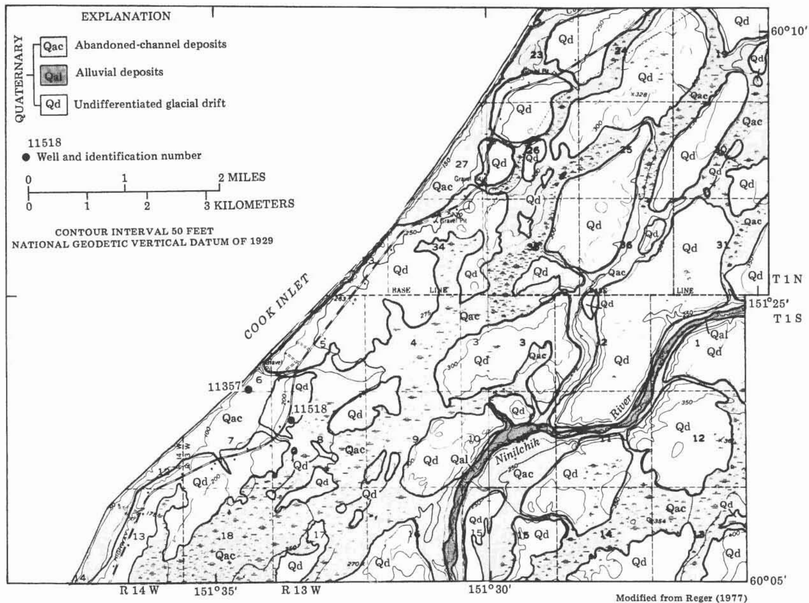
Figure 8.--Surficial geology of the upper Ninilchik River area.
