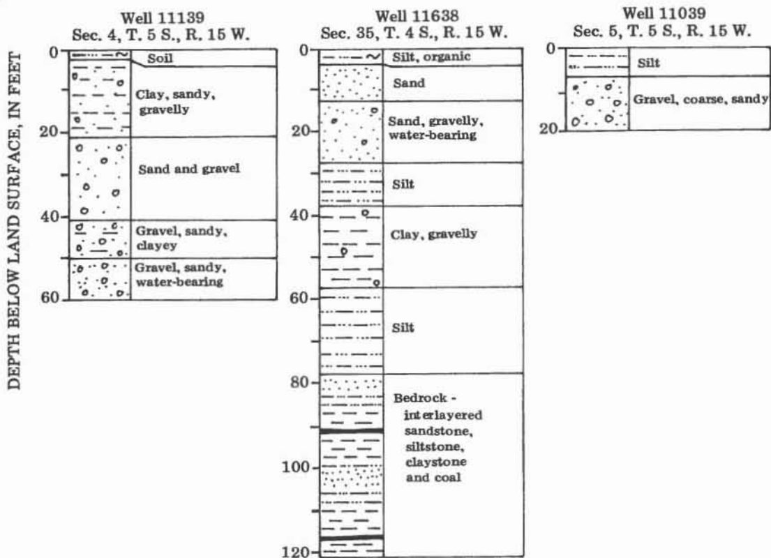
Figure 15.—Logs of selected wells in the Anchor Point area. Locations of wells are shown in figure 14.
