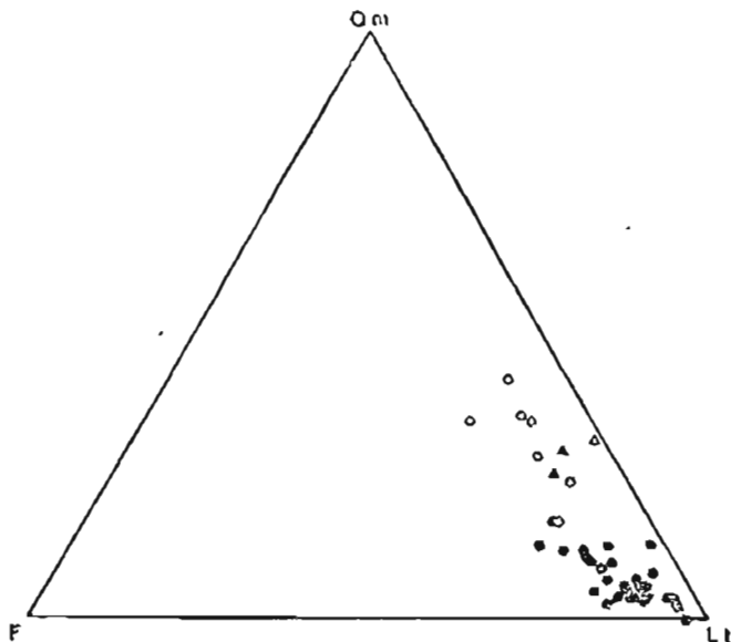
Figure 7.--Triangular QmFLt plot showing framework modes where all lithic fragments, including polycrystalline quartz, chert and quartzite fragments, are grouped with unstable lithic fragments. Qm is monocrystalline quartz; F is total feldspar; Lt is total lithic fragments. Circles are samples from the eastern area, and triangles are samples from the western area. Open circles or triangles are fine- to very fine grained samples, and solid circles or triangles are medium- to coarse-grained samples.
