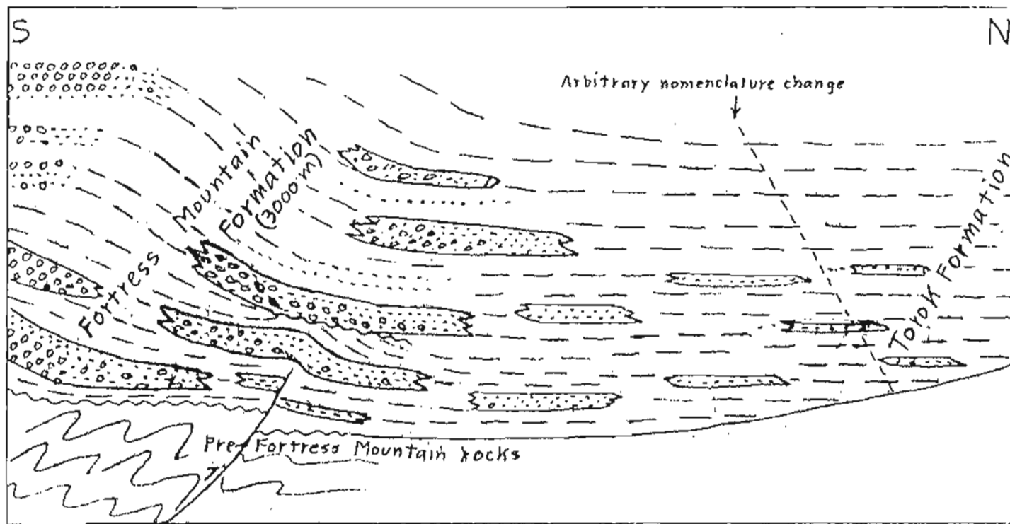
Figure 3.-Conceptual cross section across Southern Foothills showing inferred facies relations of Fortress Mountain and Torok Formations prior to intense folding. Horizontal beds in upper left are alluvial and shallow-marine facies, tilted beds are slope shales and submarine canyon facies, and lower horizontal beds are basinal shale and turbidite facies. No scale intended.
