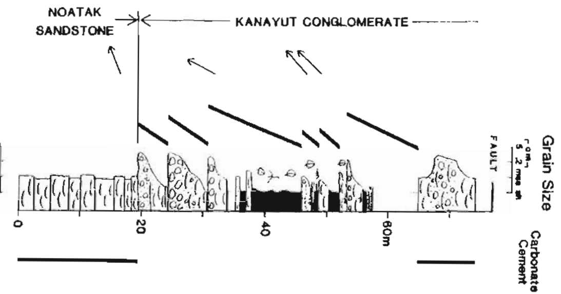
Figure 13.--Measured section of uppermost Noatak Sandstone and lower Kanayut Conglomerate at Deadlock Mountain, western Brooks Range. See Figures 1 and 9 for location of section.
