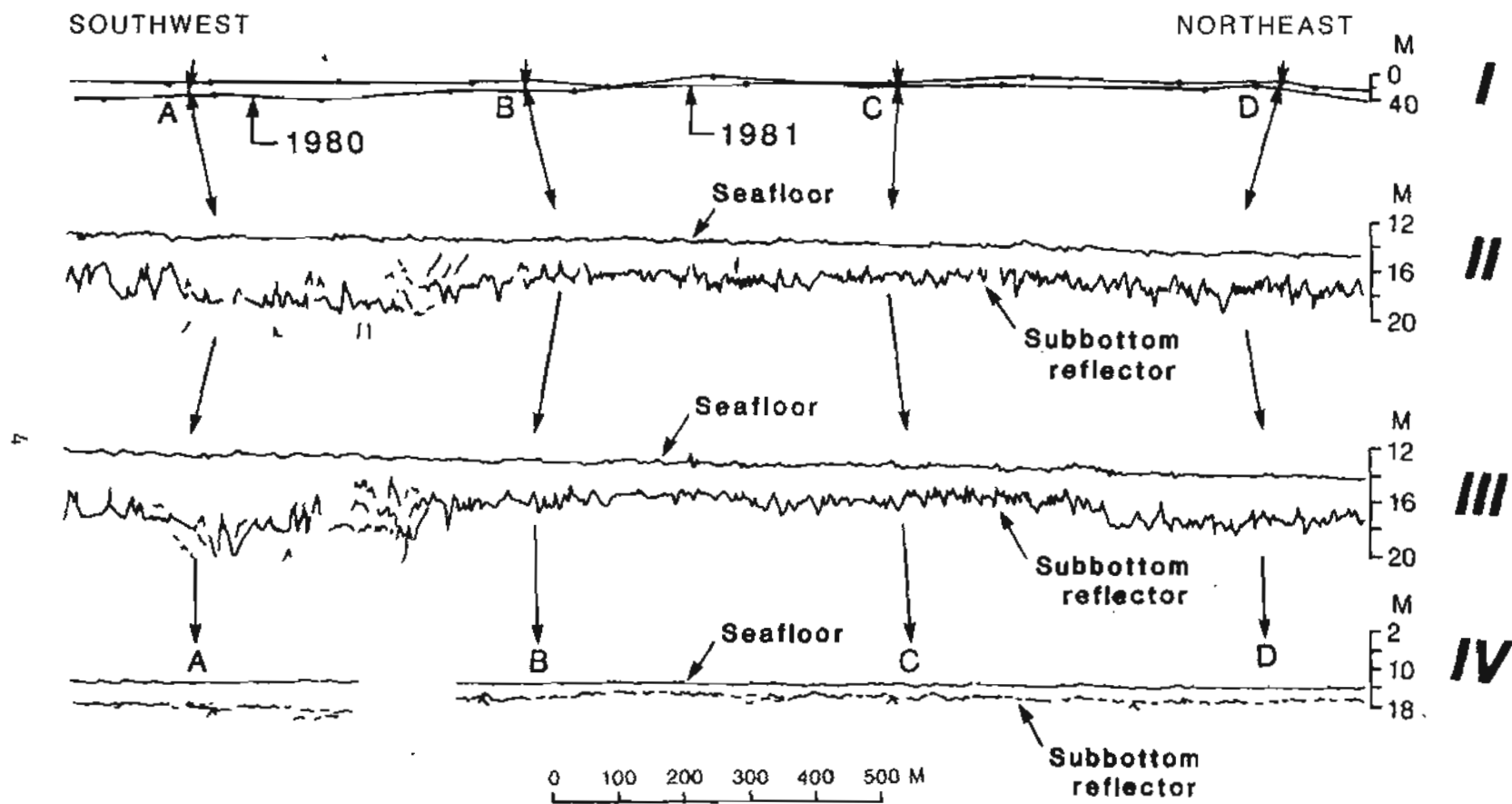
Figure 2. Trackline deviation (I) and corrections calculated from four features observed on side-scan sonar records (Fig. 3) for the years 1980 and 1981. Upper line drawing shows amount of lateral deviation along the testline between the two years. 7 kHz records (II and III) show the lack of correlation at a small scale. Boomer record (IV) shows broad scale correlation of the reflector morphology. Vertical exaggeration 20:1 on 7 kHz record and 6.6:1 on boomer record.
