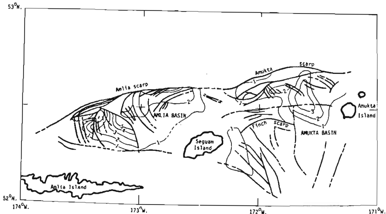
B. Isopach map of Upper Series rocks in Amia and Amukta basins. Contour interval 1 km. Modified from Geist, in prep.
