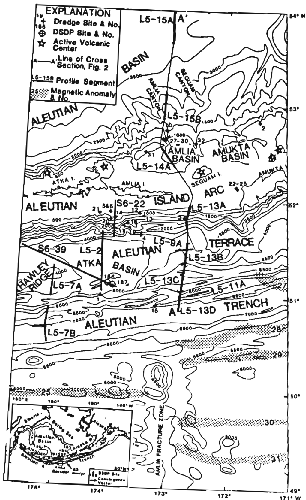
Figure 32. Map of Amlia corridor region of Aleutian Ridge and generalized cross section A-A'. From Scholl and others, 1982a.
