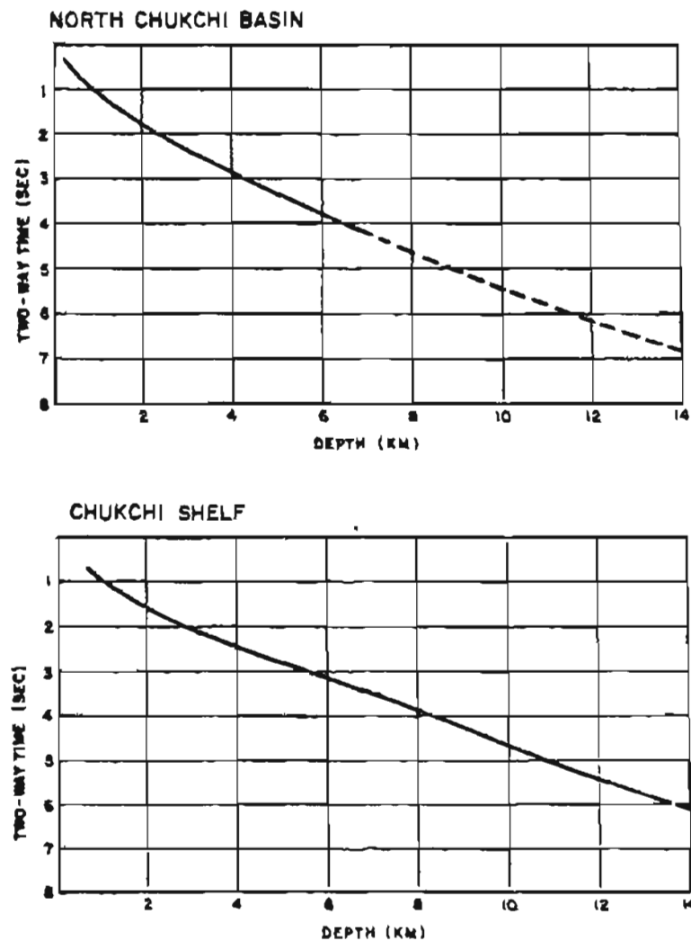
Figure 8. Explanation of map symbols in Figure 9 and plots of average seismic-reflection time as a function of depth for the Chukchi shelf and North Chukchi basin.
