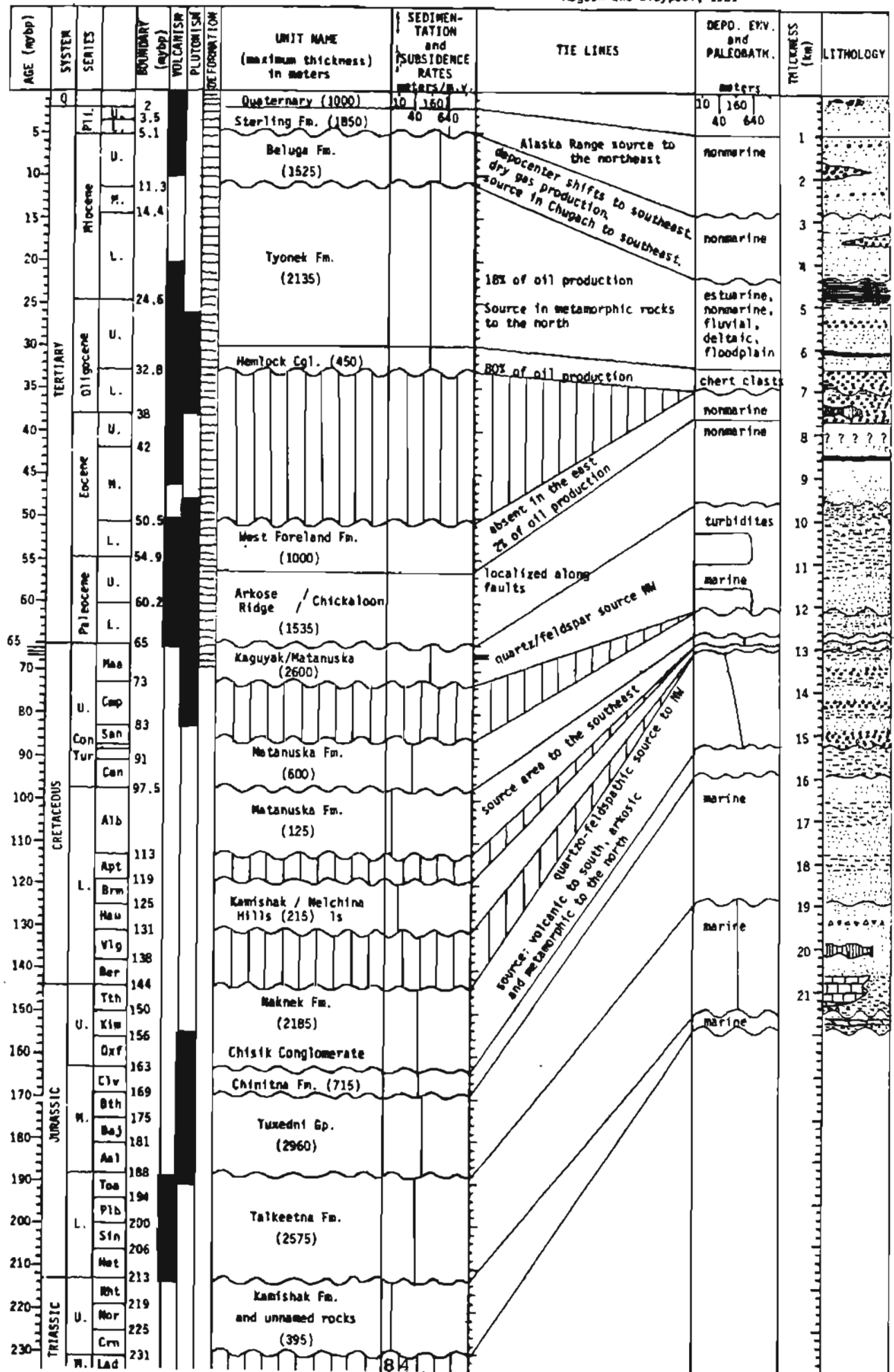
Data from Fisher and Magoon, 1978; Kirschner and Lyon, 1973; Magoon and others, 1980; and Magoon and Claypool, 1981
