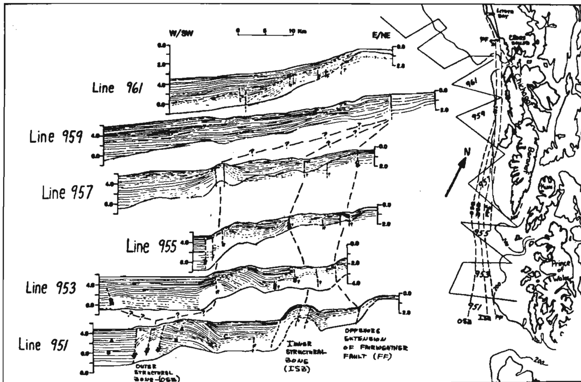
Figure 60. Generalized location of structural trends and line drawings of seismic profiles from the Southeastern Alaska segment. From Bruns, 1982a.
