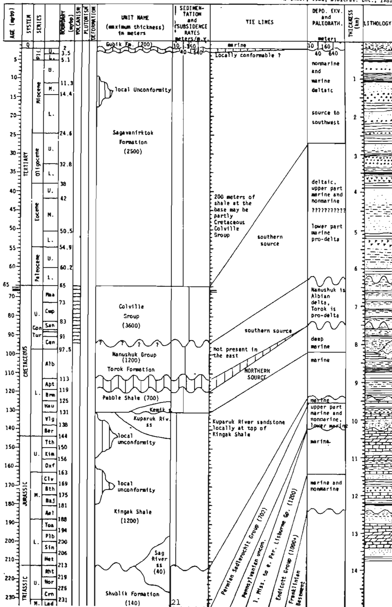
Data from Grantz and others, 1981; Molenaar, 1983; Blostrat. Cht., 1981
