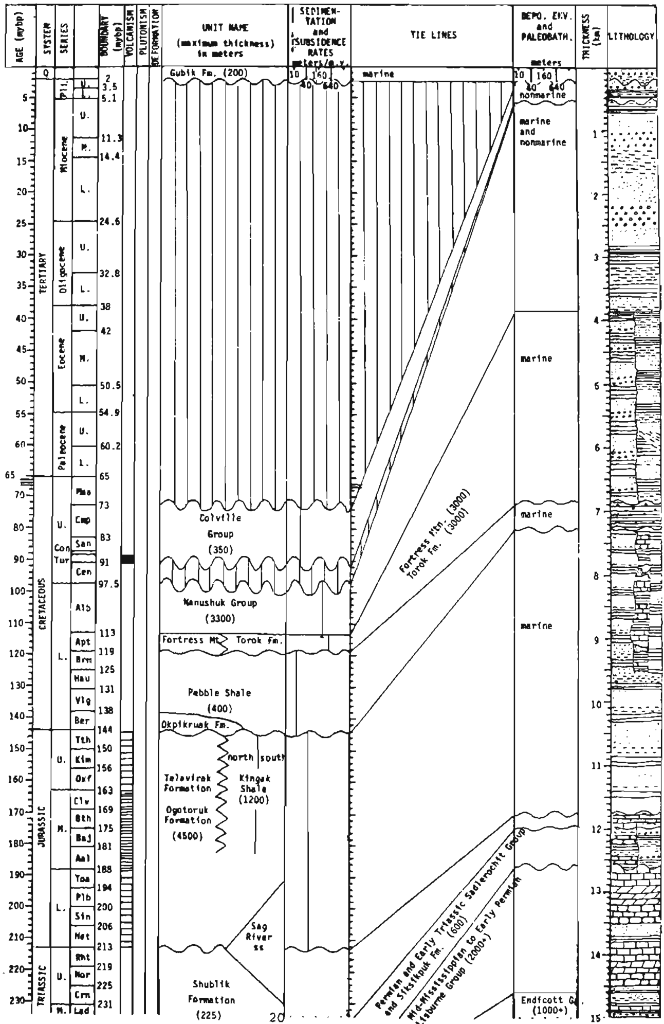
Data from Grantz and others, 1981; North Slope Biostrat. chart, 1981
