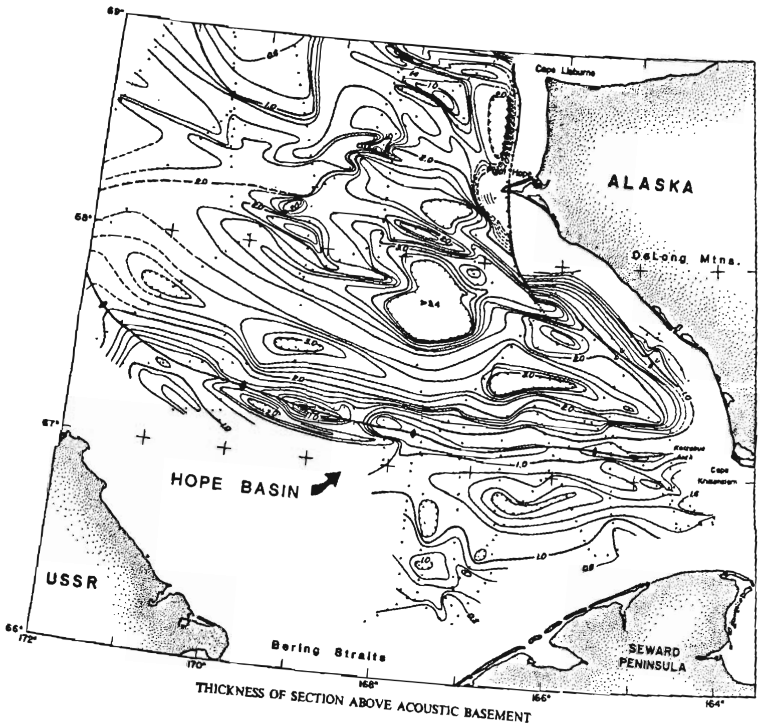
Figure 16. Isopach map of Hope basin. Contour interval 0.2 kilometers. From Eittreim and others, 1978.
