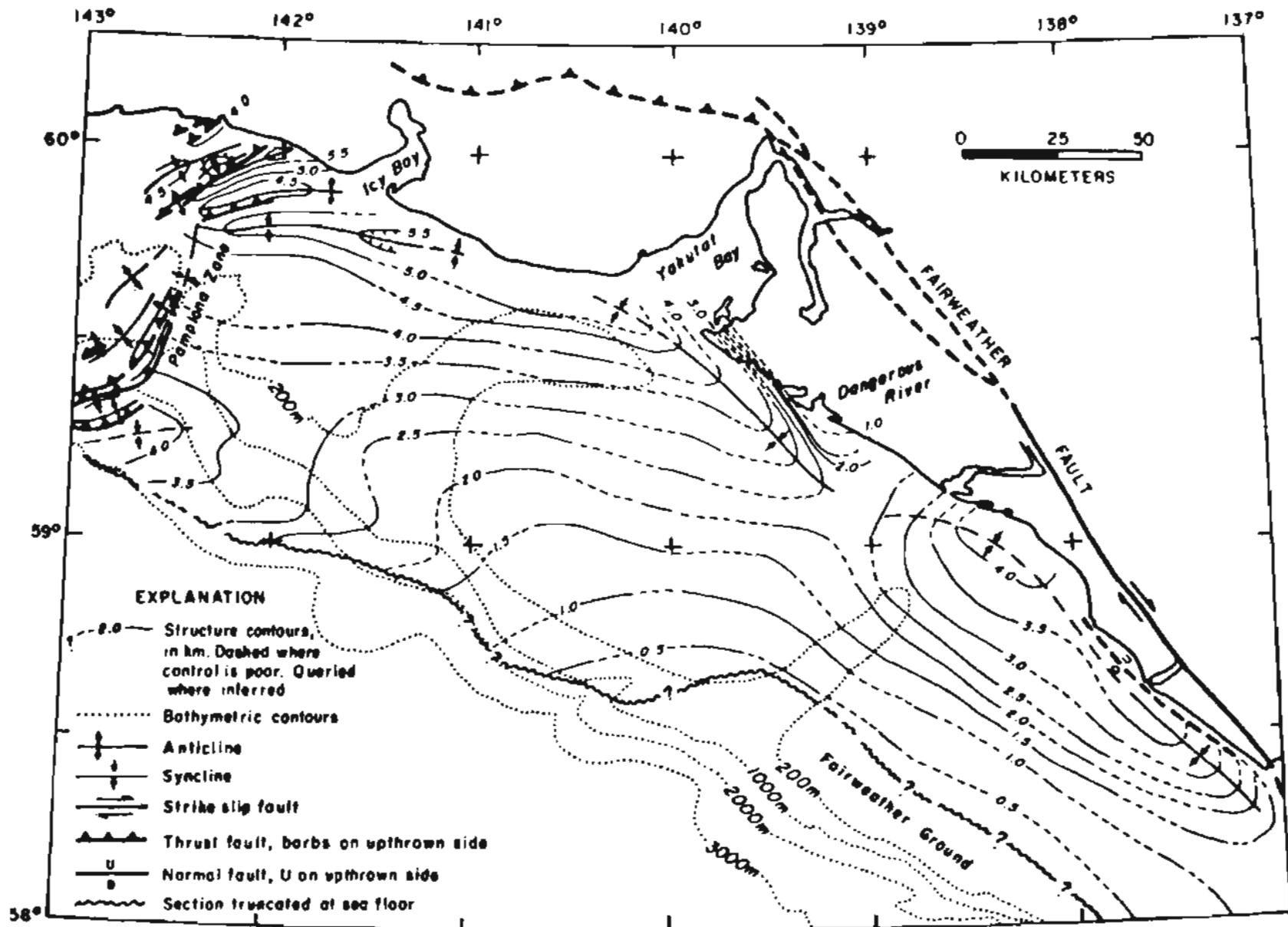
Figure 57. Structure-contour map of the Yakutat segment of the Gulf of Alaska basin. Contours on a seismic horizon at approximately the base of Neogene sedimentary strata. From Bruns, 1982a.
