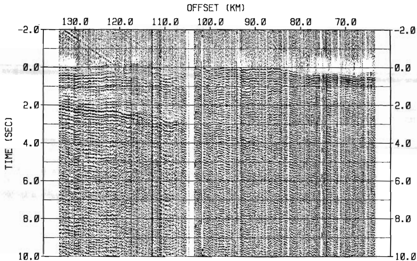
Figure 28 Profile 1 Shot 11 Shot Point 132 AGC = 2 sec
