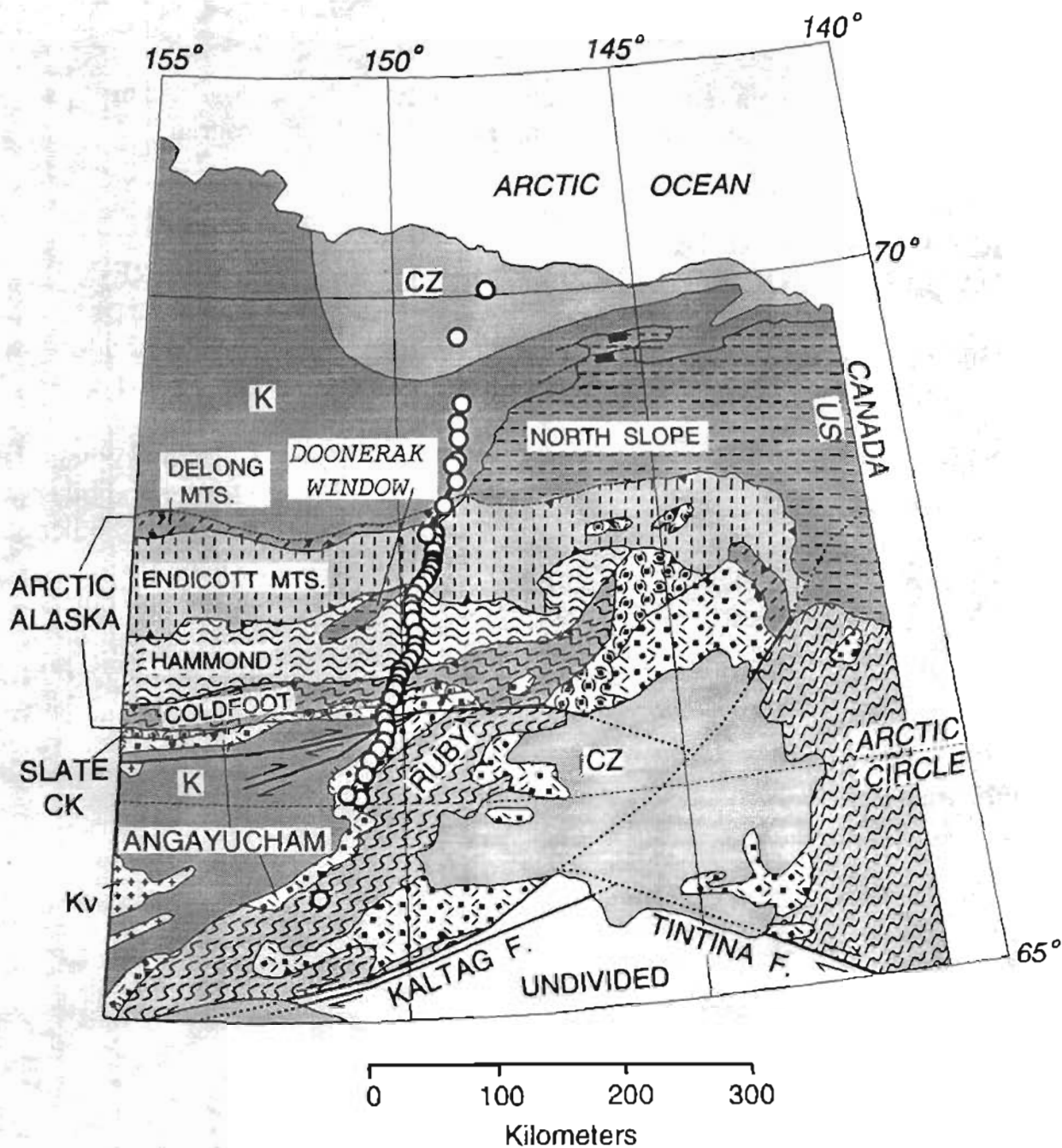
Figure 2. Experiment location map, showing terranes and subterrane. Circles represent shotpoint locations. From south to north terranes include the Ruby, Angayucham, Slate Creek, and Arctic Alaska terranes. Subterrane of the Arctic Alaska terrane include the Coldfoot, Hammond, Endicott Mts., Delong Mts. and North Slope subterrane.
