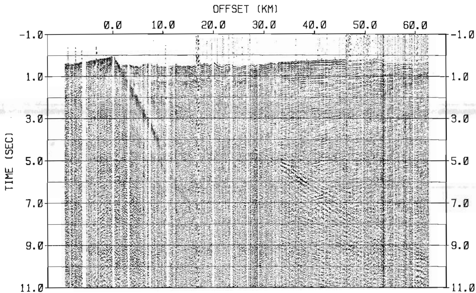
Figure 32 Profile 2 Shot 13 Shot Point 127 AGC = 2 sec
