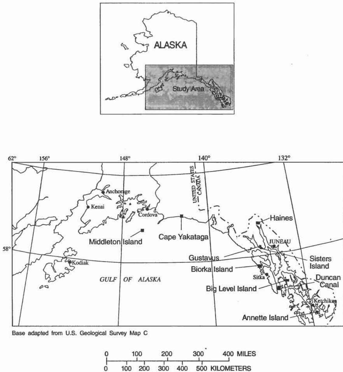
Figure 1. Location of nine coastal and island sites in south-central and southeast Alaska.
