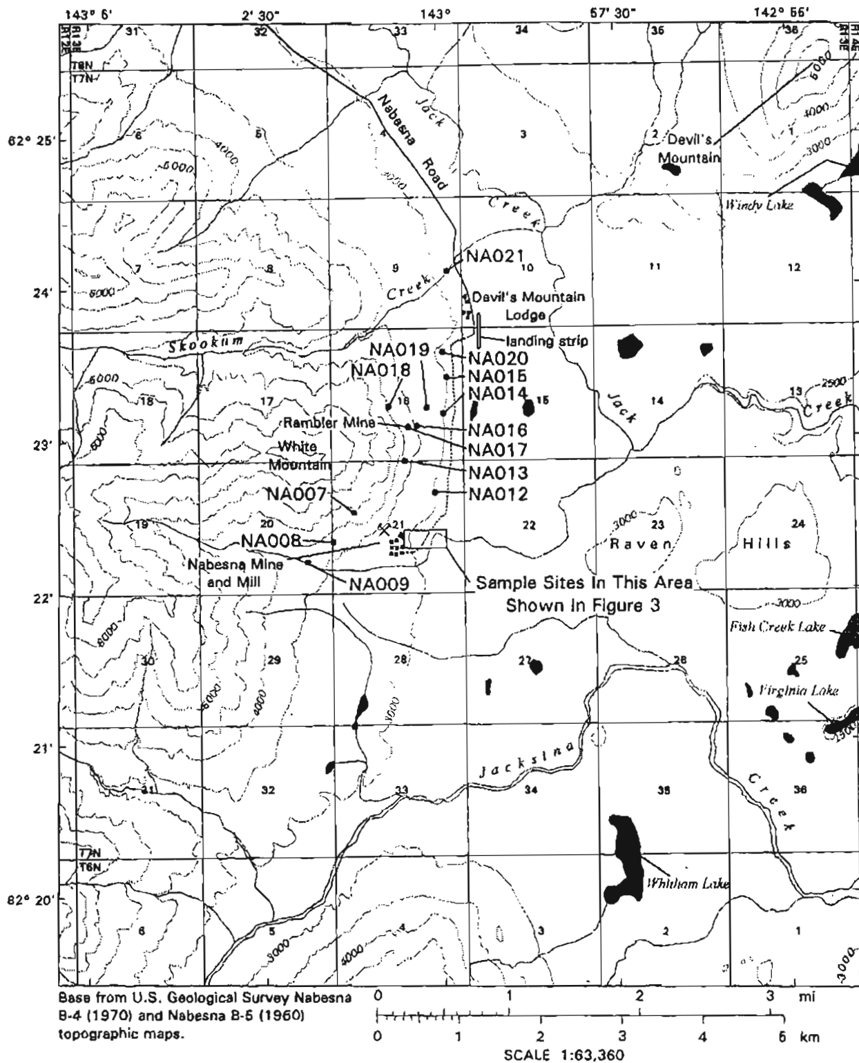
Figure 2. Site locations for samples collected in the Nabesna mine area, Alaska.
