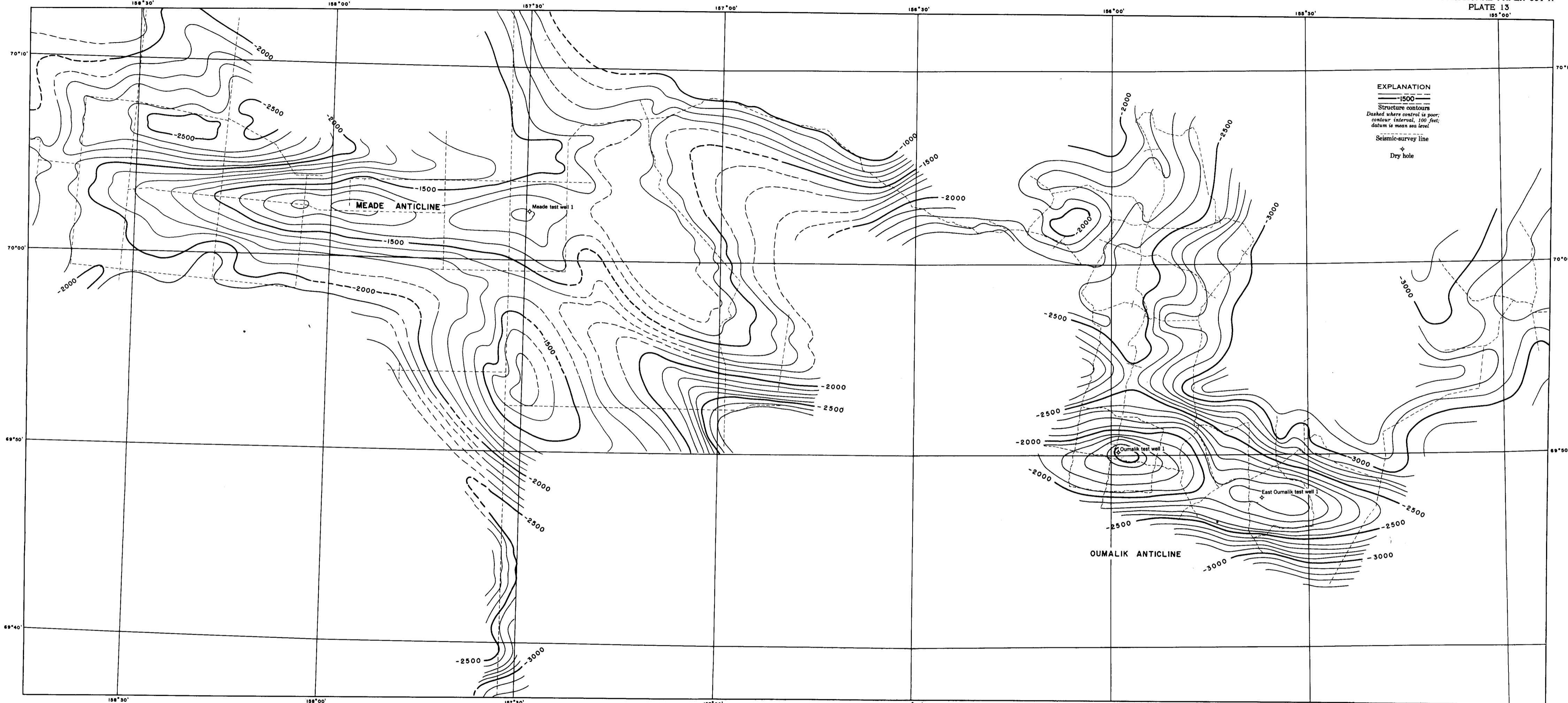
STRUCTURE- CONTOUR MAP OF SHALLOW LOWER CRETACEOUS ROCKS, MEADE AND OUMALIK ANTICLINES, NORTHERN ALASKA
