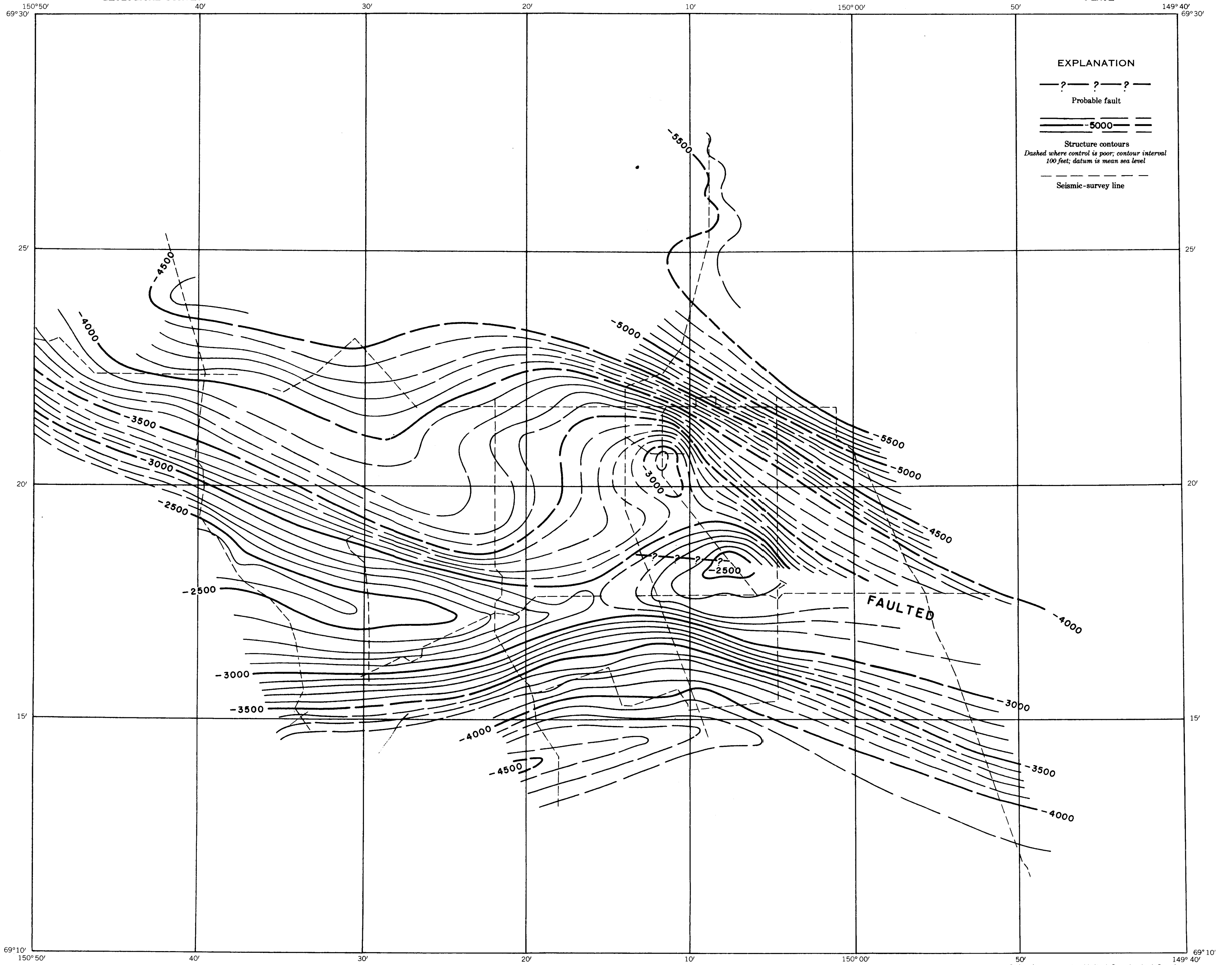
STRUCTURE-CONTOUR MAP OF THE KUPARUK ANTICLINE, CONTOURED ON A SEISMIC HORIZON IN CRETACEOUS ROCKS, NORTHERN ALASKA
