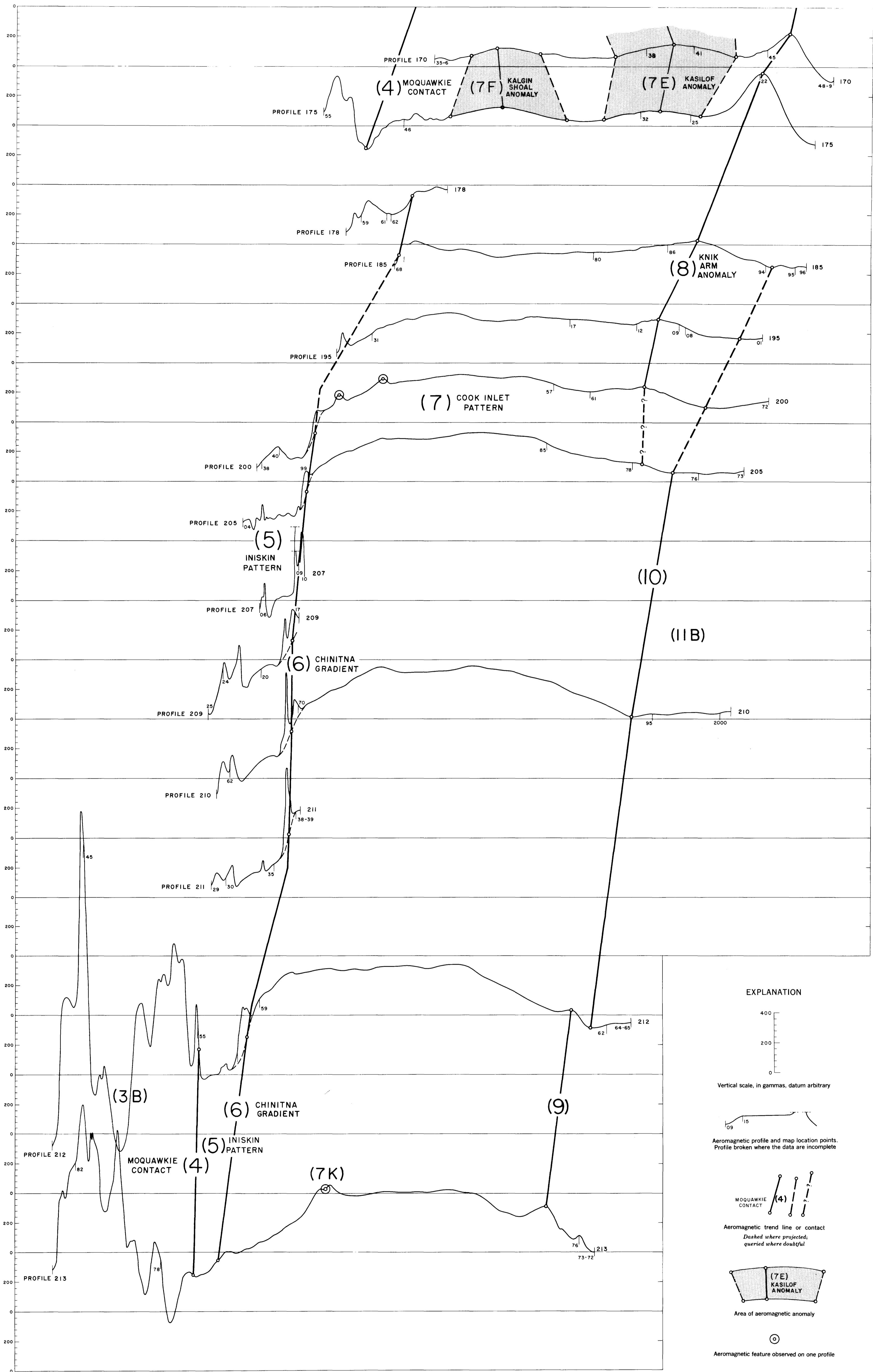
TOTAL INTENSITY AEROMAGNETIC PROFILES OF THE SOUTHERN COOK INLET AREA, ALASKA, FLIGHT LINES 170 TO 213 PROFILES NOT ADJUSTED TO A COMMON DATUM POSITION OF FLIGHT LINES AND MAP LOCATION POINTS SHOWN ON PLATE 18
