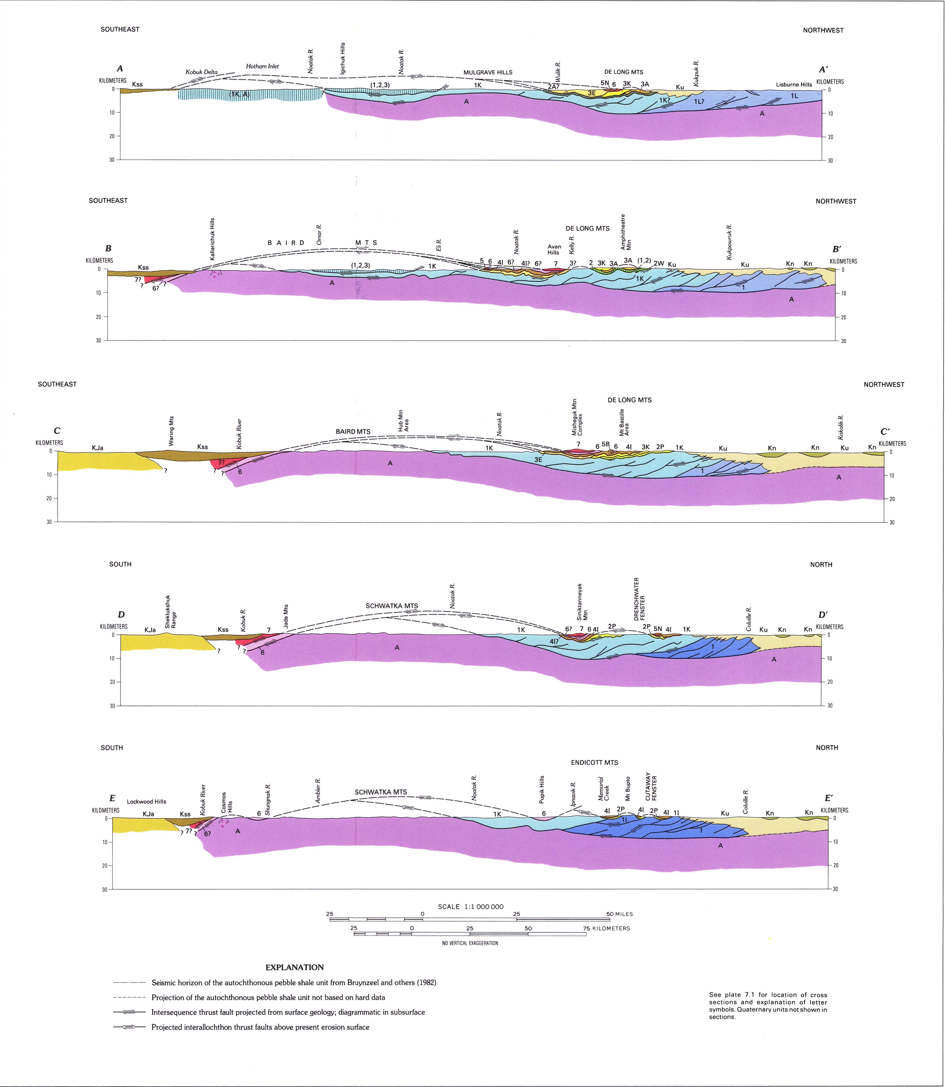
CROSS SECTIONS OF THE WESTERN BROOKS RANGE, ALASKA
