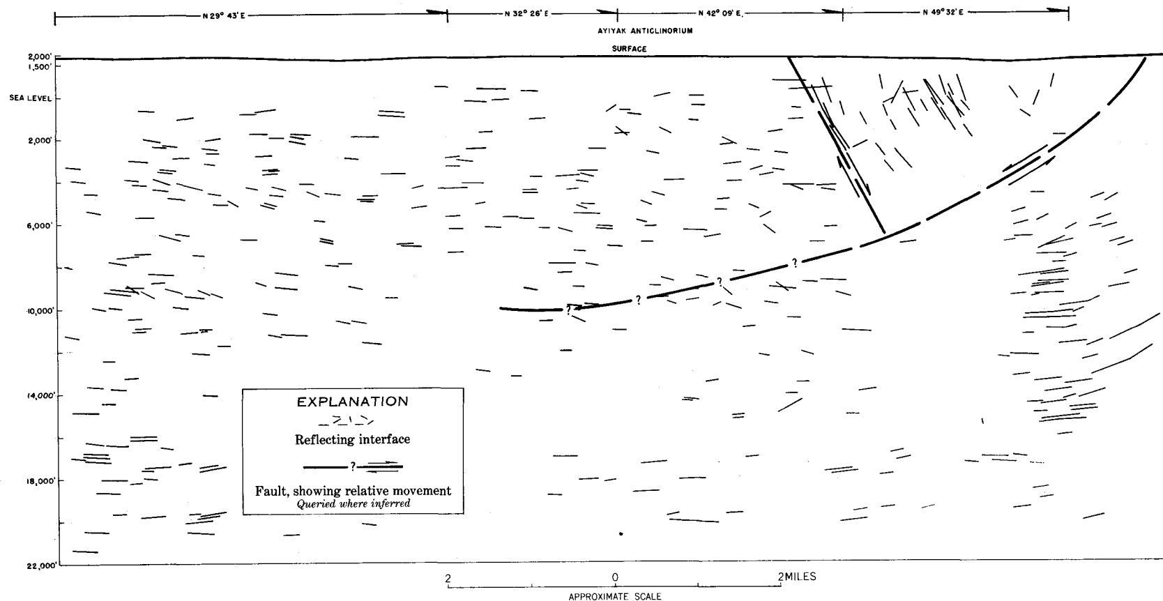
FIGURE 4.—Diagrammatic section of Ayiyak anticlinorium, Castle Mountain area.
