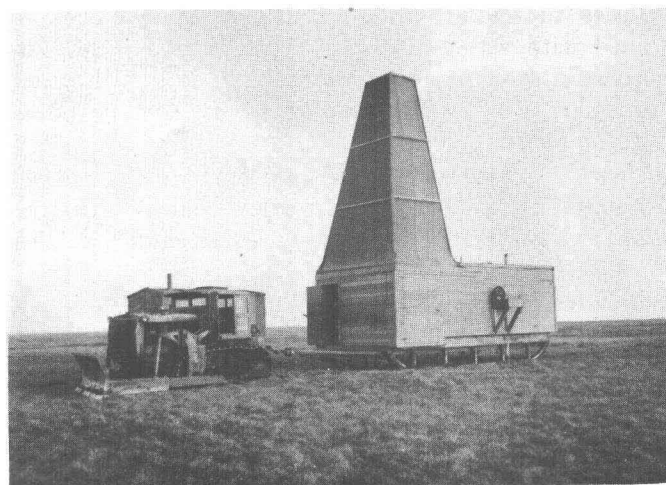
B. Seismograph drill and tractor party.
