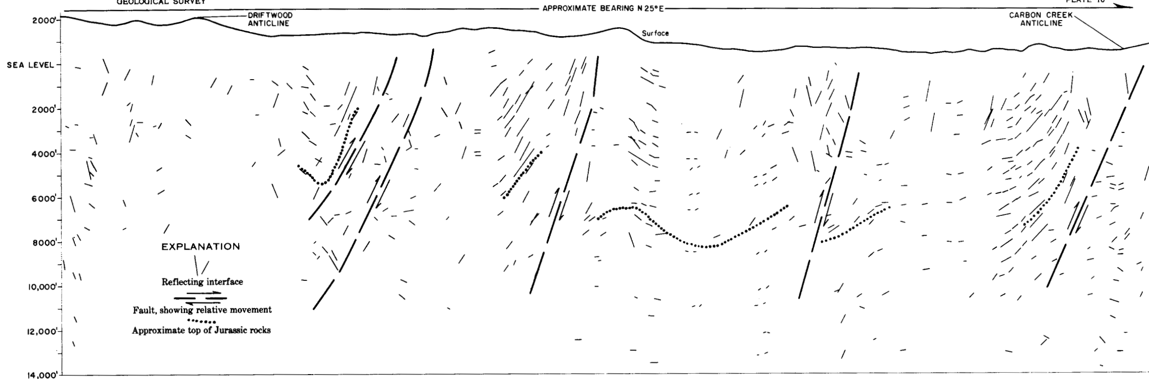
DIAGRAMMATIC SECTION BETWEEN CARBON CREEK AND DRIFTWOOD ANTICLINES, NORTHERN ALASKA
