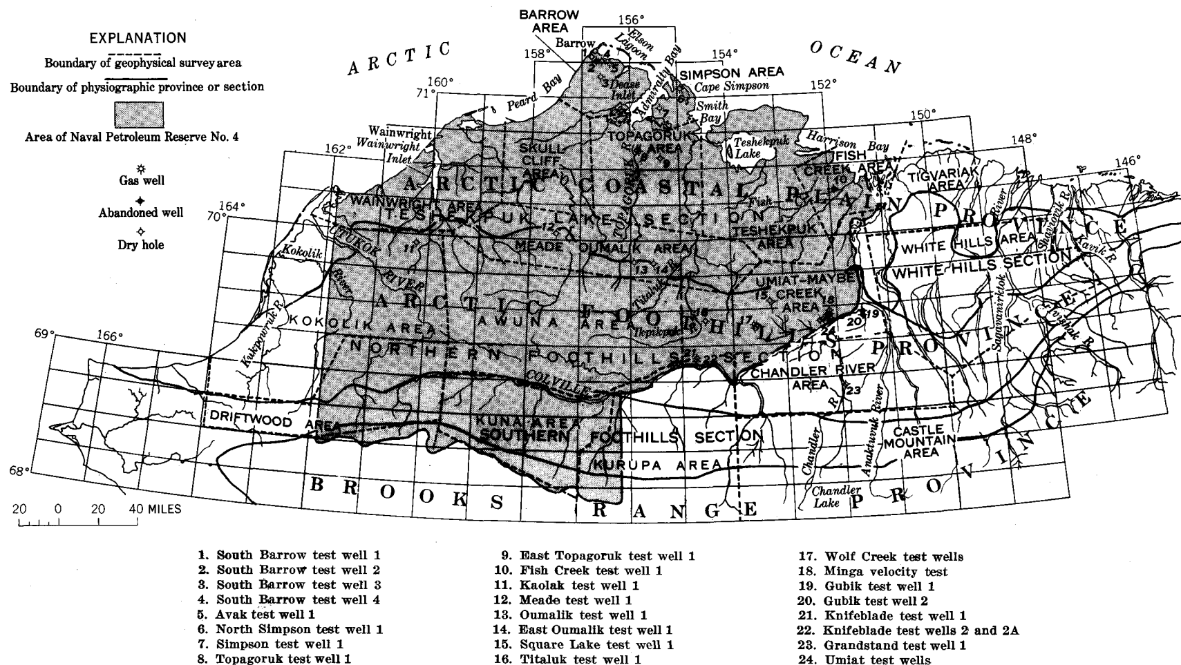
FIGURE 1.—Index map of northern Alaska showing designation of areas of geophysical surveys. Numbers indicate location of wells listed.
