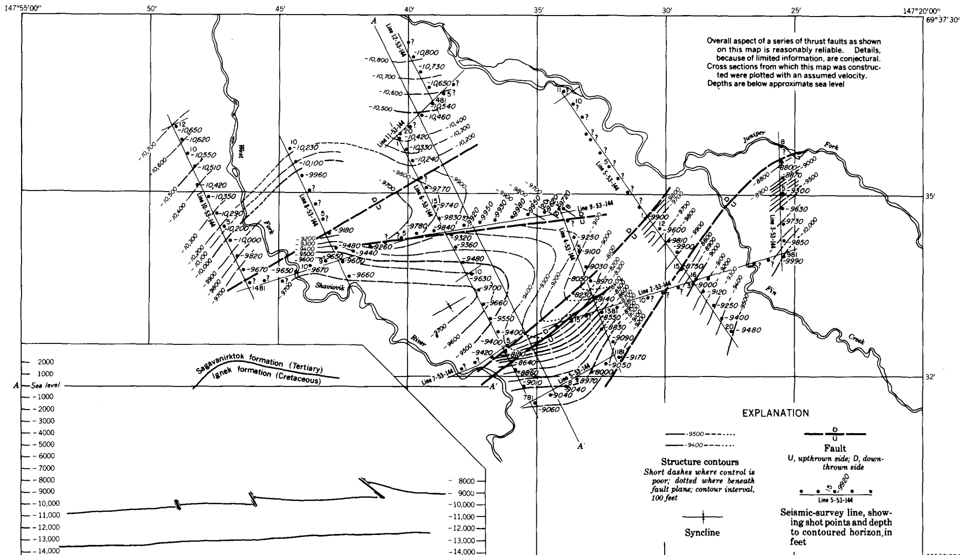
STRUCTURE-CONTOUR MAP OF INTERMEDIATE REFLECTING ZONE, SHAVIOVIK AREA, NORTHERN ALASKA
