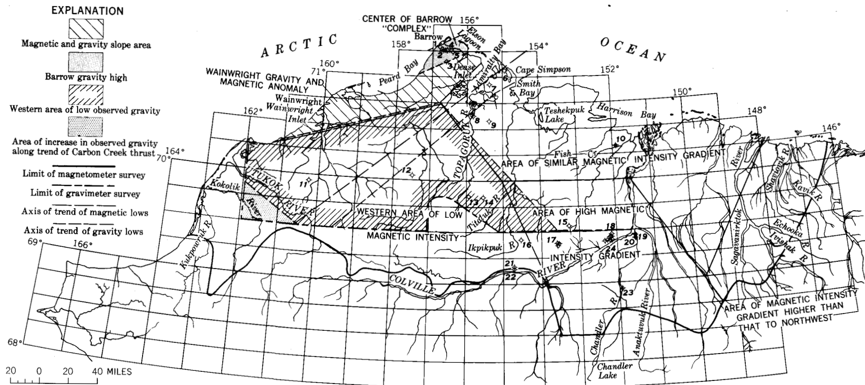
FIGURE 3.—Limits of magnetic and gravity surveys and outlines of anomalous areas. Numbers indicate wells listed on figure 1.
