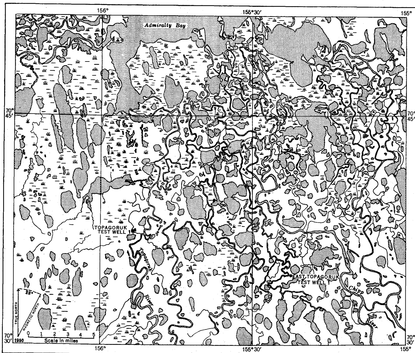
FIGURE 15.—Map showing location of Topogoruk test well 1 and East Topogoruk test well 1.
