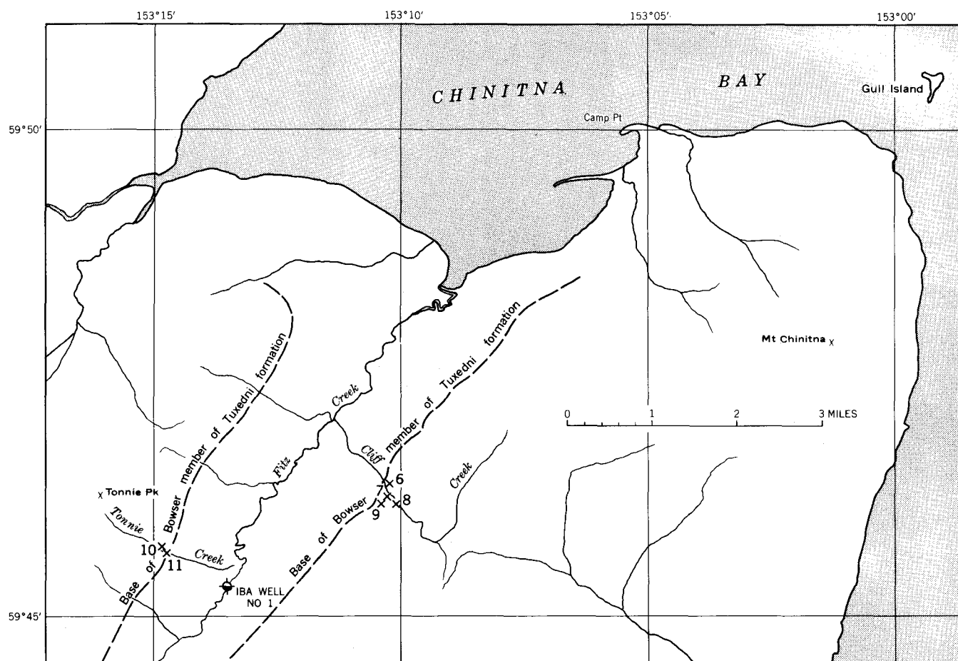
FIGURE 4.—Index map showing occurrences of upper Bajocian (Jurassic) fossils in the northern part of the Iniskin Peninsula. (Numbers on map refer to those given in the locality list (table 2) and in the distribution table.)
