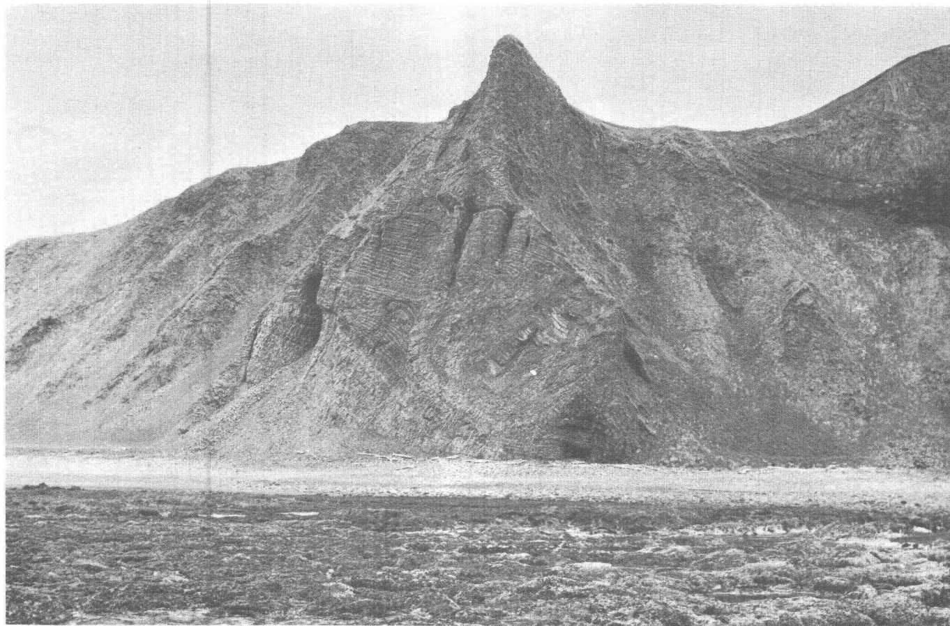
FIGURE 11.—Layered albited dacite lava pod in sea cliff west of Buttress Point, Unalaska Island. Rocks in wave-cut rock bench in foreground and steep cliff above layered lava in center of picture are pillowd lava. Dark argillite strata and a massive sill show in upper right. Figure 12 is a closeup of the layered lava at the base of the sea cliff just left of the small cave shown in the center of the photograph.
