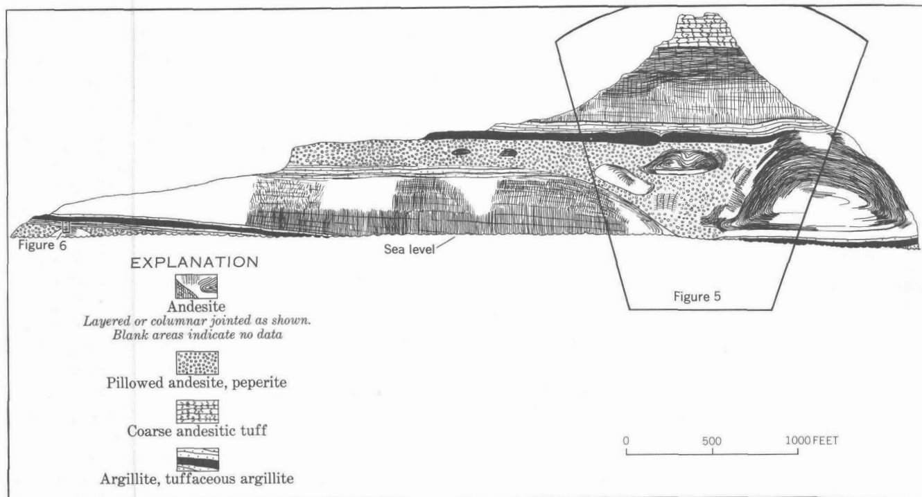
FIGURE 4.—Sketch showing geologic relations in sea cliffs on south and southwest sides of Tower Point, Unalaska Island; drawn from a series of photographs. Overlapping areas of figures 5 and 6 shown by insets. Lava pod on right, also shown in Drewes and others (1961, fig. 86), is the largest one known with completely exposed concentric layering.
