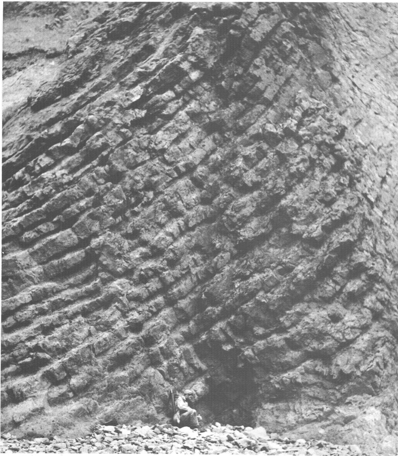
FIGURE 9.—Layered albitized dacite in active sea cliff on east side of Buttress Point, Unalaska Island. Upper contact of lava pod against small lens of tuffaceous sediment shown in upper left of photograph; for detail see figure 10. Photographed from the same place as figure 8 but from the opposite direction.
