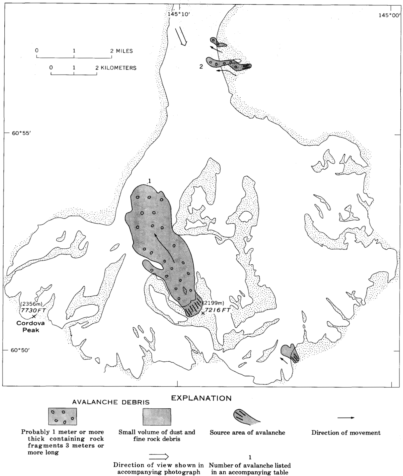
FIGURE 9.—Map of rockslide avalanche on Schwan Glacier.
