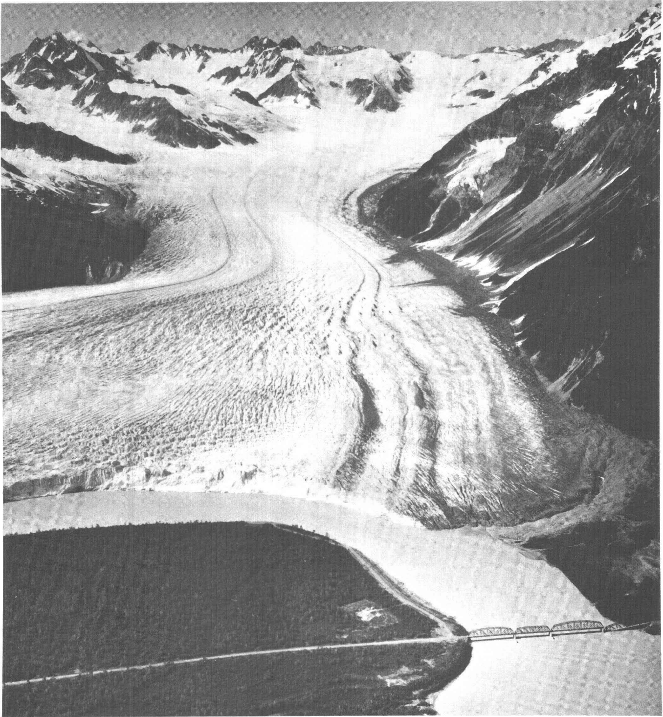
FIGURE 20.—Childs Glacier, August 25, 1965, showing conditions after the earthquake. The size and distribution of the small rockslides on the glacier are fairly typical of the slides in many areas in the Chugach and Kenai Mountains. No dynamic response of the glacier to these avalanches has been noted, nor, in view of the small volume of the rockslides, is a response probable. Since 1960, this glacier has thickened and advanced in the terminal area. Note the change in the glacier on the right; the small marginal lakes visible in the 1963 view are almost completely covered by the advancing glacier in 1965. The Million Dollar Bridge, a span of which was shaken down by the earthquake, crosses the Copper River (lower right of the photograph).
