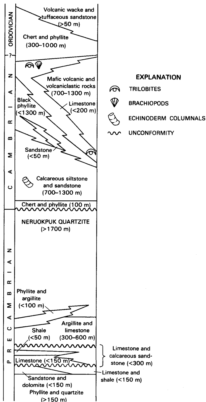
FIGURE 2.—Generalized stratigraphic relations among Precambrian and early Paleozoic rocks, northeastern Brooks Range, based on information from Reiser and others (1980). Base not exposed; younger rocks present at top of section but not shown.
