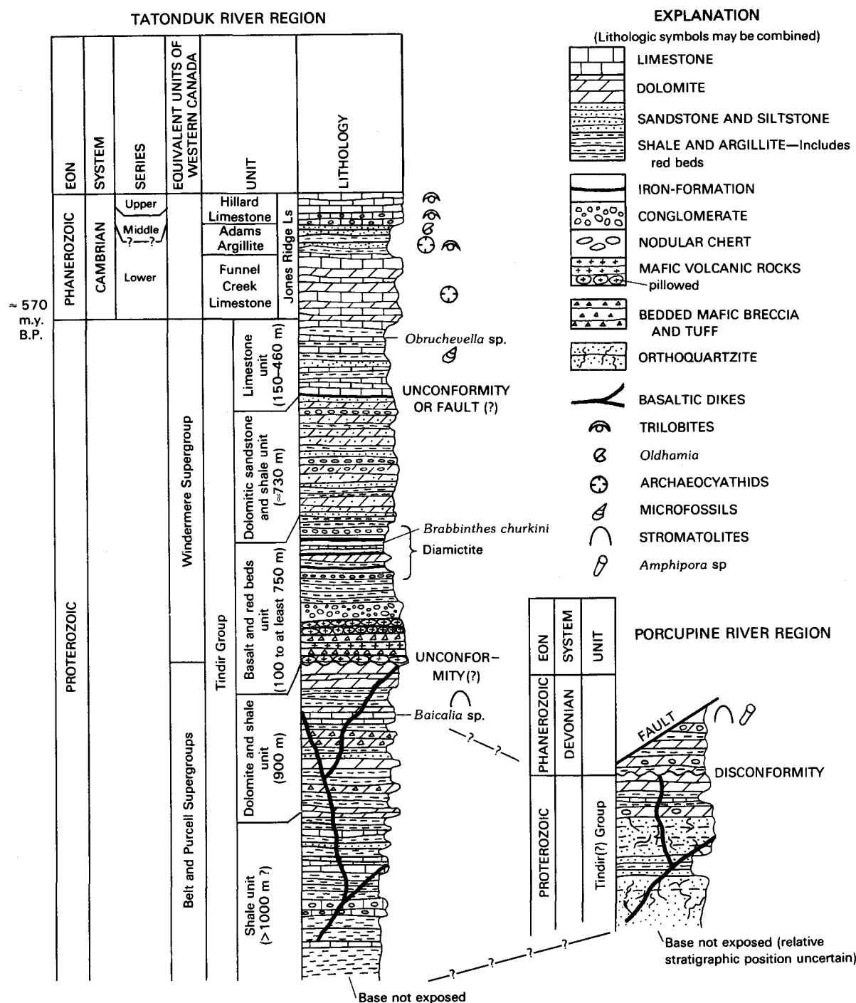
FIGURE 3.—Generalized composite columnar sections of the Tindir Group, east-central Alaska. Tatonduk River region modified from Mertie (1933) and Brabb and Churkin (1965, 1969). Porcupine River region modified from Brosgé and others (1966).
