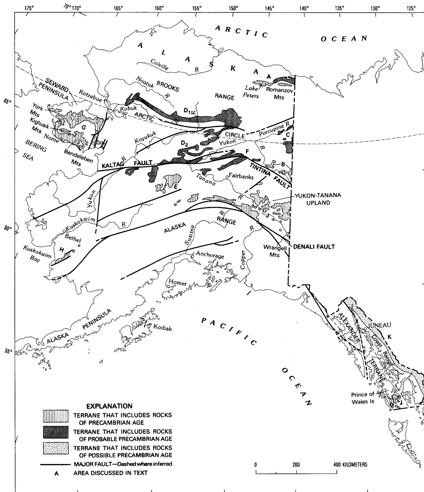
FIGURE 1.—Distribution of Precambrian, probable Precambrian, and possible Precambrian rocks in Alaska. A, northeastern Alaska; B, east-central Alaska (Yukon River region); C, east-central Alaska (Porcupine River region); D 1 and D 2 , west-central Alaska (Yukon-Koyukuk region and southern Brooks Range); E, central Alaska (northeastern Kuskokwim Mountains); F, central Alaska (Livengood-Crazy Mountains region); G, Seward Peninsula; H, southwestern Alaska; I, southernmost southeastern Alaska; J, east-central Alaska (Yukon-Tanana upland); K, southeastern Alaska (Coast Range).
