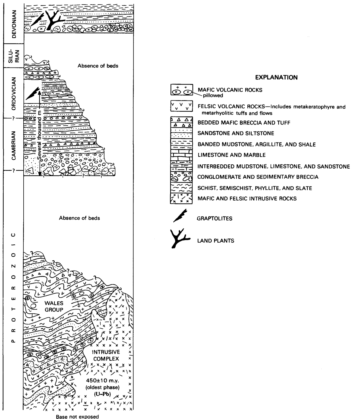
FIGURE 4.—Generalized stratigraphic relations of the Wales Group, southeastern Alaska. Queries in section indicate uncertainty of extent and stratigraphic and structural relations of discontinuous deposits. Modified from Churkin and Eberlein (1977).
