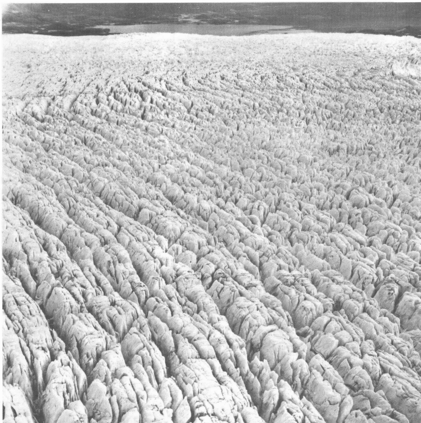
FIGURE 2.—Oblique aerial photograph showing roughness of the glacier surface. The major crevasse valleys are about 20 m deep and 50 m apart. The center of the scene is about 2.5 km upglacier from the terminus, view to southeast. The glacier flows from left to right. U.S. Geological Survey photograph No. 75M5-56, by L. R. Mayo, October 8, 1975.
