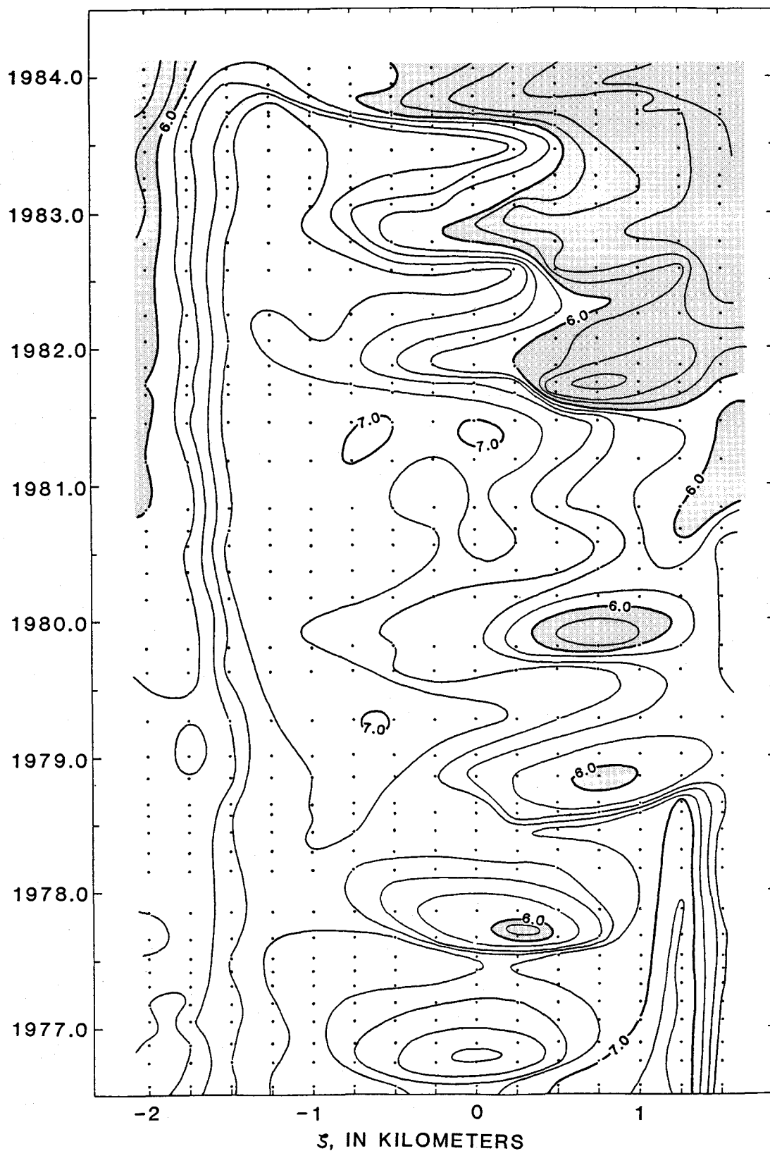
FIGURE 10.—Diagram showing position of the terminus Z as a function of transverse distance \xi and time. The contoured variable is the amount (in kilometers) by which the distance from the head of the glacier exceeds 60 km; area with values less than 6.0 (66.0 km) are stippled. The approximate western border of the terminus is along the left margin of the diagram; the eastern border of the terminus is to the right of the right margin.
