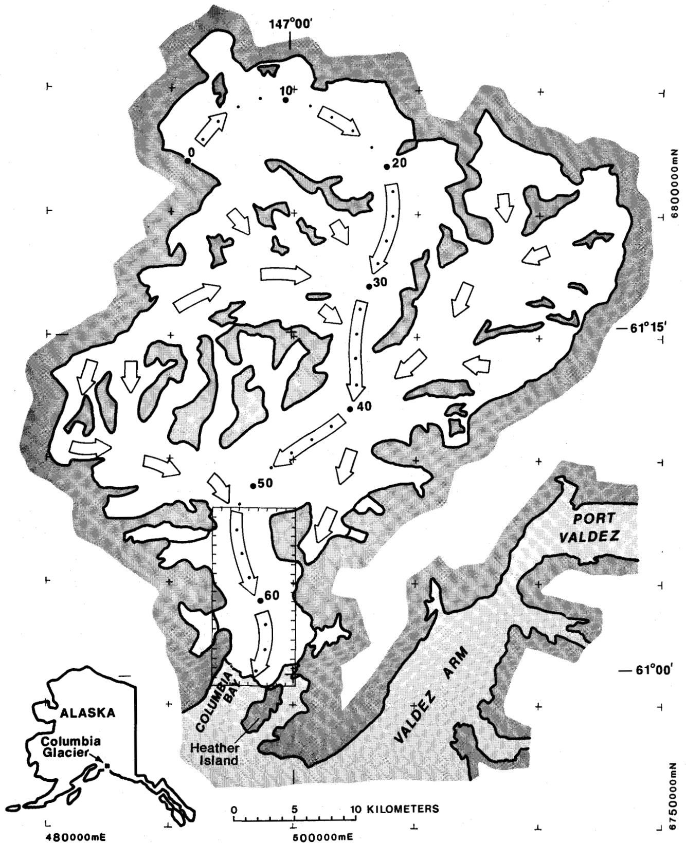
FIGURE 1.—Columbia Glacier, Alaska. Arrows show the direction of flow; longer arrows indicate the main ice stream. Dots are at 2-kilometer intervals along the \xi -axis. The box marks the section of the square ( \Delta x = \Delta y = 762.5 m) data grid consisting of (horizontal) rows 51–71, numbered from north to south, and of (vertical) columns 18–27, numbered from west to east.
