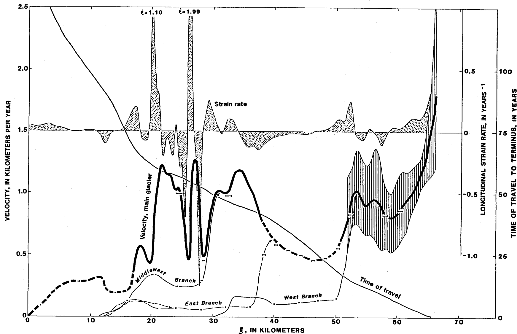
FIGURE 13.—Velocity along the centerline during the measurement year as a function of longitudinal distance for the main glacier (heavy) and its tributaries (light, dashed). For the main glacier, the time of travel to the terminus (light) and the longitudinal strain rate (stippled) are shown, as is the range of velocity variations with time in the lower reach (striped). Velocity values derived by stake surveys are shown as short lines indicating displacements during the year. Note: Stake at \xi \approx 33 km was not on exact centerline.
