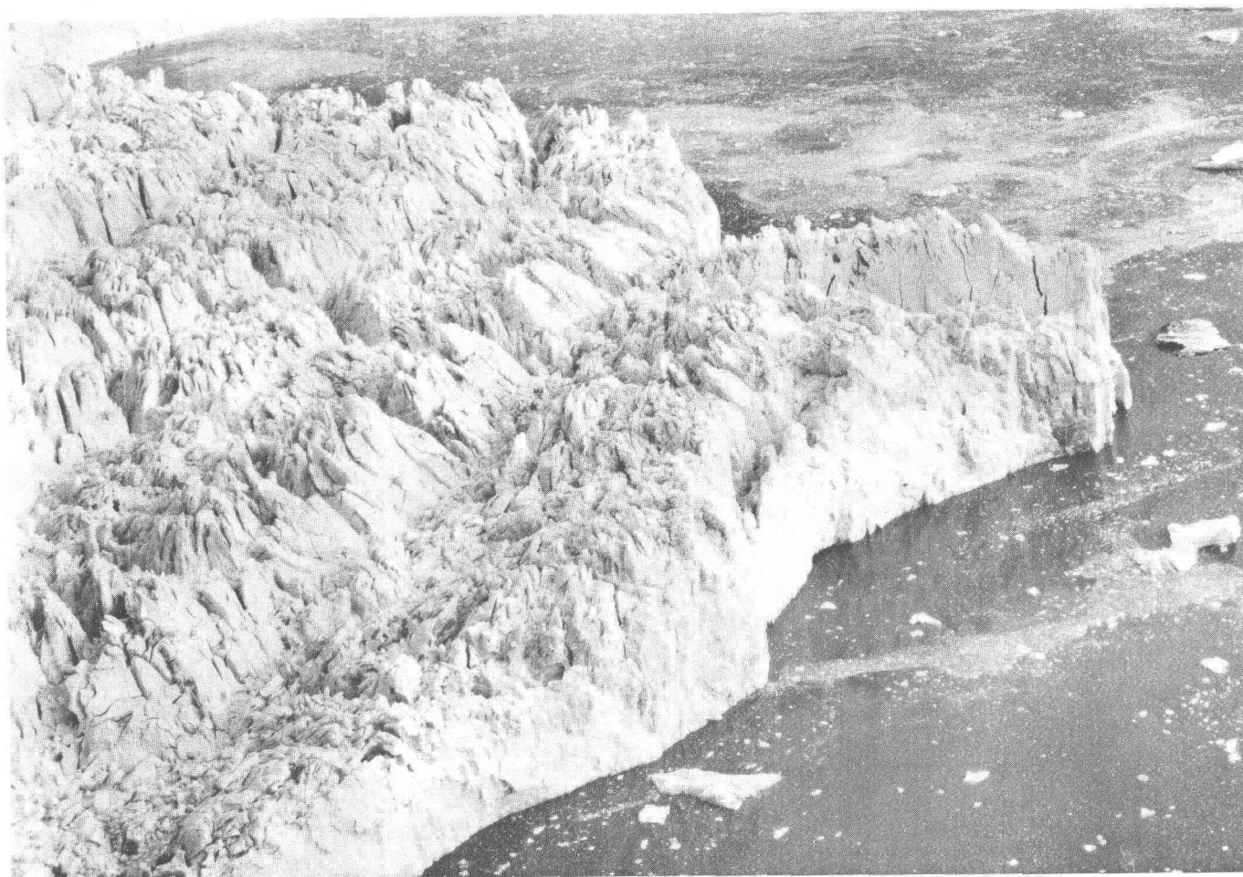
FIGURE 9.—Oblique aerial photograph of a part of the terminus, showing rough surface near the terminus ice cliff, October 8, 1975. U. S. Geological Survey photograph No. 75M5-54, by L. R. Mayo.
