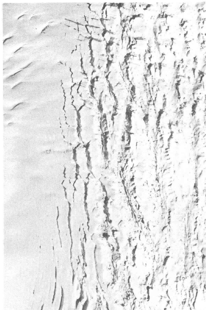
FIGURE 17.—Vertical aerial photograph of the main glacier in the vicinity of \xi=26 km, April 29, 1978, showing marked increase in crevasse width over a short distance due to intense extension. The glacier flows to the right (south).
