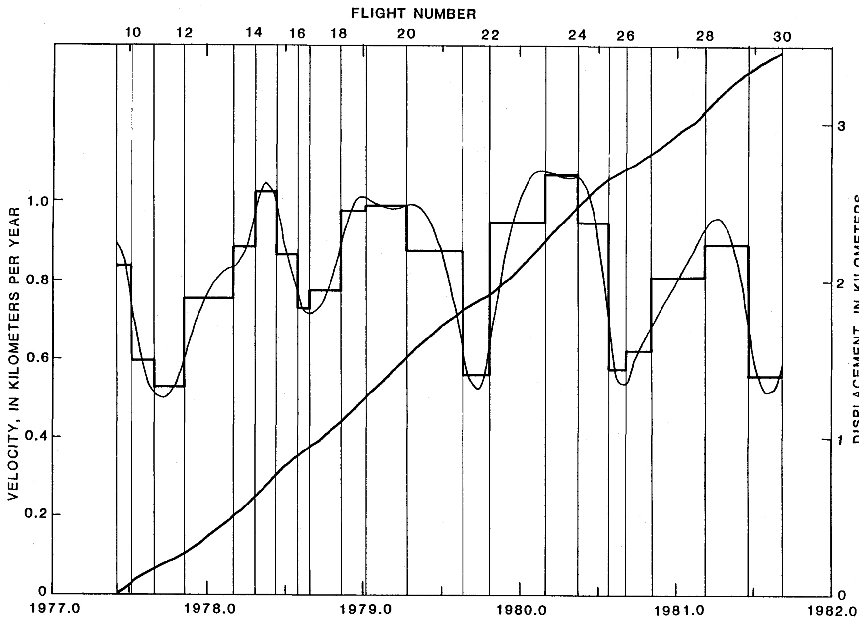
FIGURE 18.—Cubic spline (heavy) through pseudotrajectory points (eq. 8, scale at right) and the quadratic spline velocity function (light, scale at left) obtained from it, for row i=60 , over the period June 2, 1977 through September 1, 1981 (flights 9 through 30). Also shown (step function) are the average velocity values V_L between successive flight dates.
