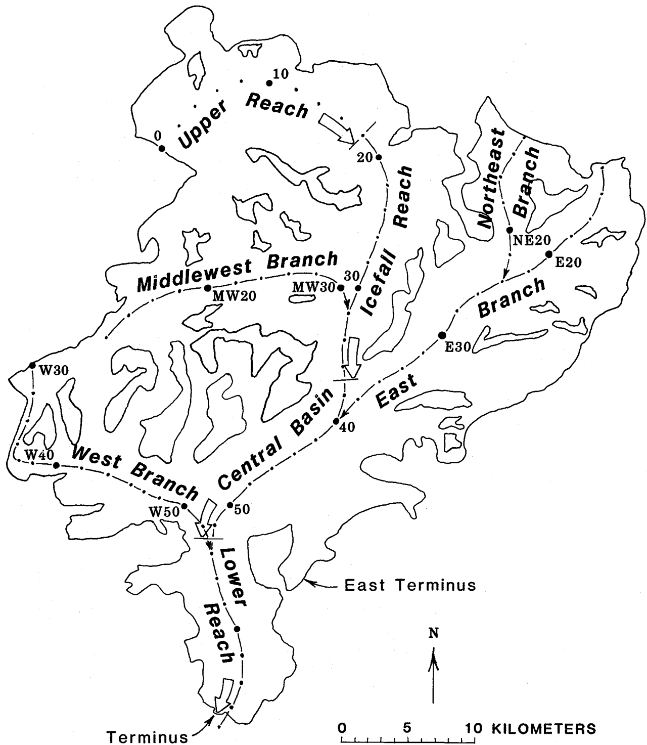
FIGURE 6.—Columbia Glacier, showing longitudinal ( \xi ) coordinates and informal names of several reaches and tributaries.
