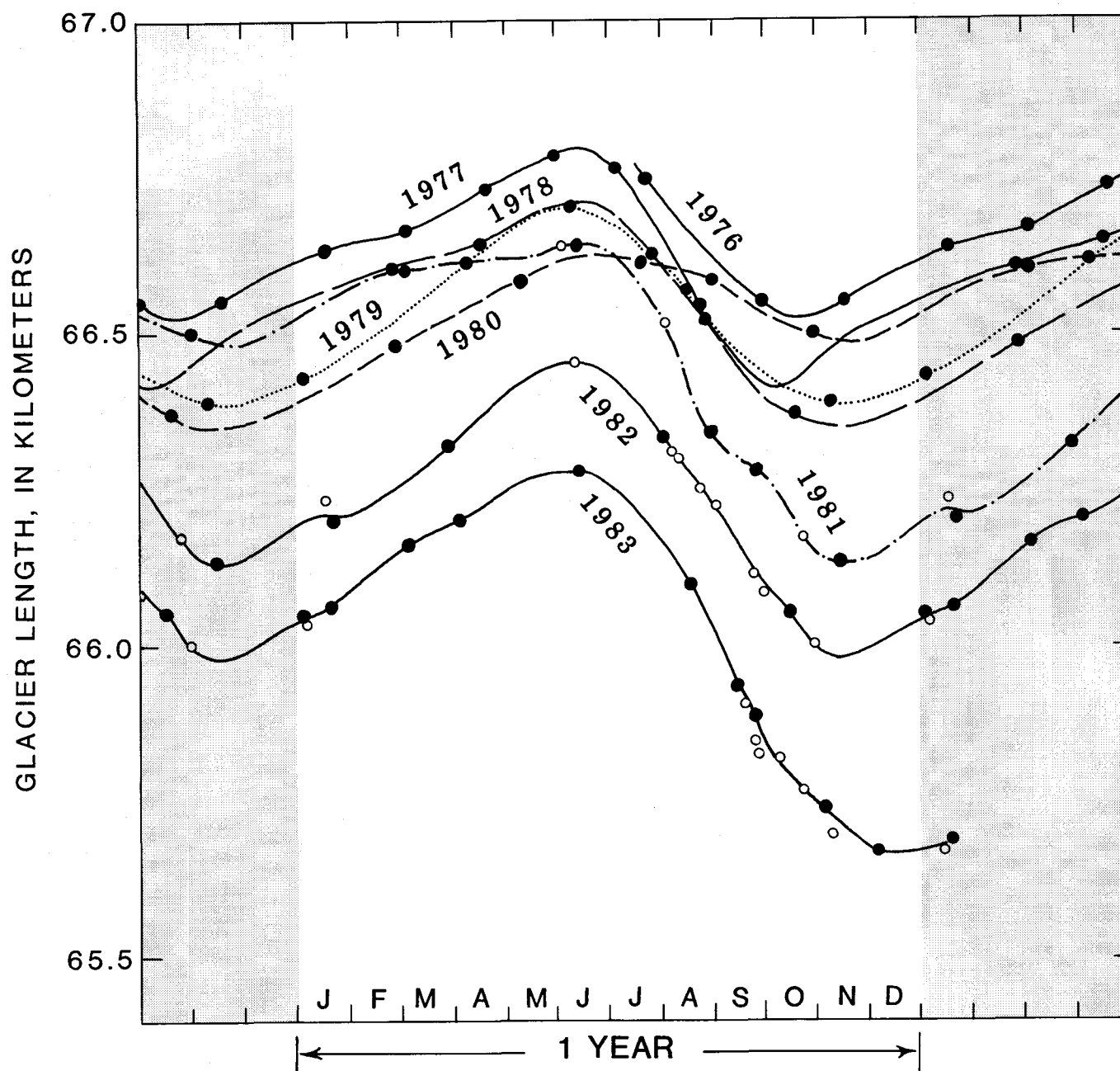
FIGURE 12.—Seasonal advance and retreat of Columbia Glacier for the years 1976–83, superimposed onto one year for comparison. The curves are repeated to either side in the gray areas to help visualize trends. Solid dots are data points obtained by photogrammetry (error is about 10 m), open circles are observations by less accurate methods (ship-borne radar, ground surveys), and the lines are smooth curves drawn through data points. Values are averaged over the width of the active terminus.
