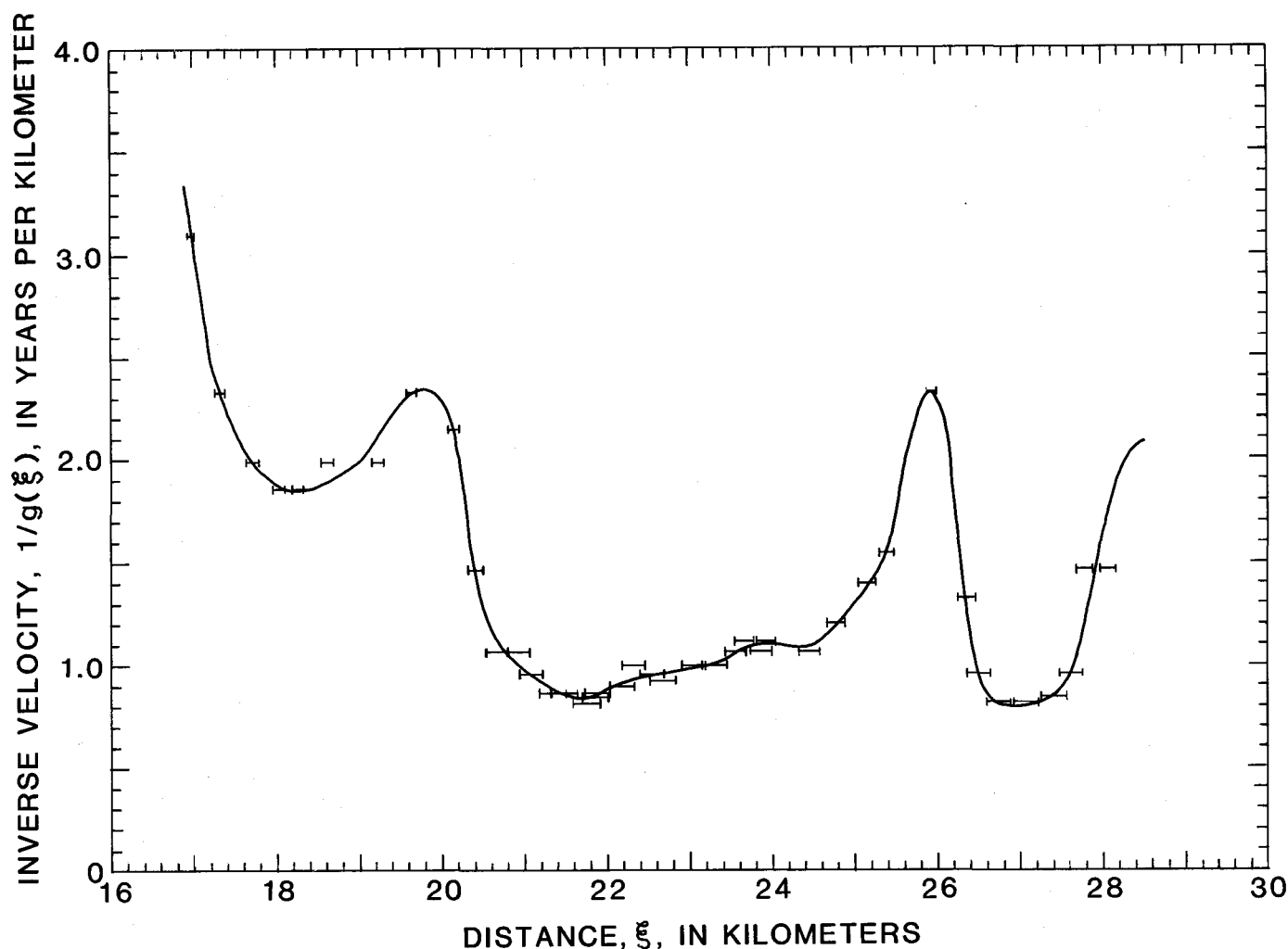
FIGURE 14.—Velocity-reciprocal function 1/g(\xi) in the icefall reach. The integral conditions (eq. 3) imposed by particle trajectory endpoints are also shown; they are met, in a least squares sense, by the curve.
