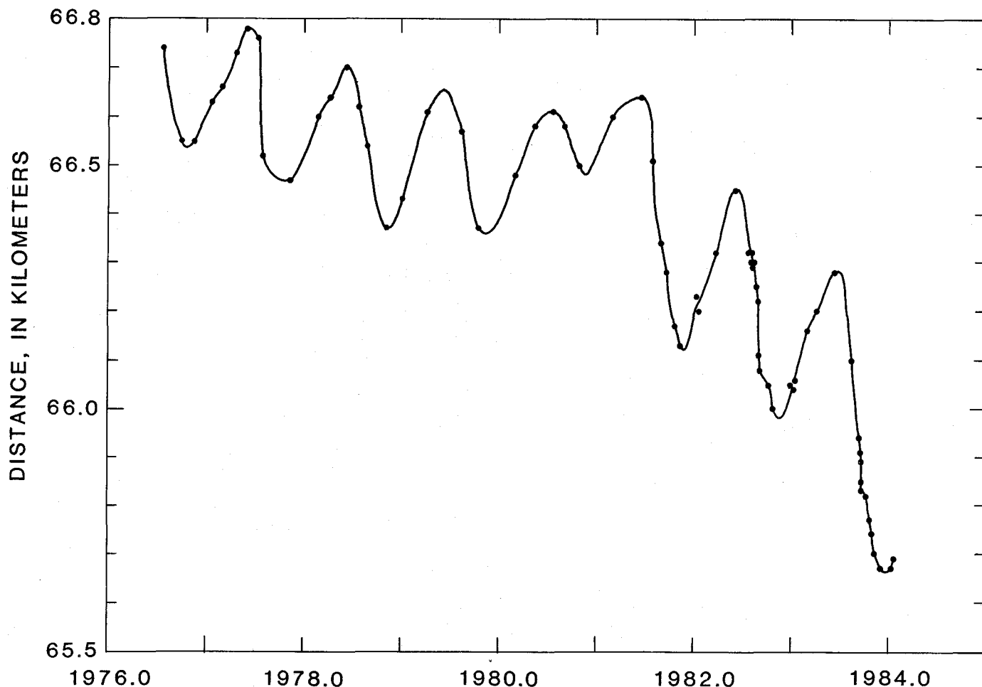
FIGURE 11.—Hand-drawn curve through width-averaged terminus position \langle \Xi \rangle as a function of time for the flights 3–45 (table 2).
