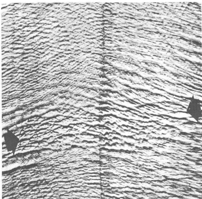
FIGURE 7.—Superimposed portions of vertical aerial photographs illustrating the photograph-overlay method. The two photographs, taken on September 26 and November 15, 1981, are displaced about 190 m in the north-south direction. Note that in an area between the two arrows the image appears sharp, whereas above and below that, the image area appears doubled and confused. The sharp area marks a zone of constant displacement (velocity). North is to the top, and flow is from top to bottom. This area of the glacier is about 950 m wide and is located near the center of the glacier at \pm 64.4 km. The vertical dark band is a streak of debris on the ice (medial moraine).
