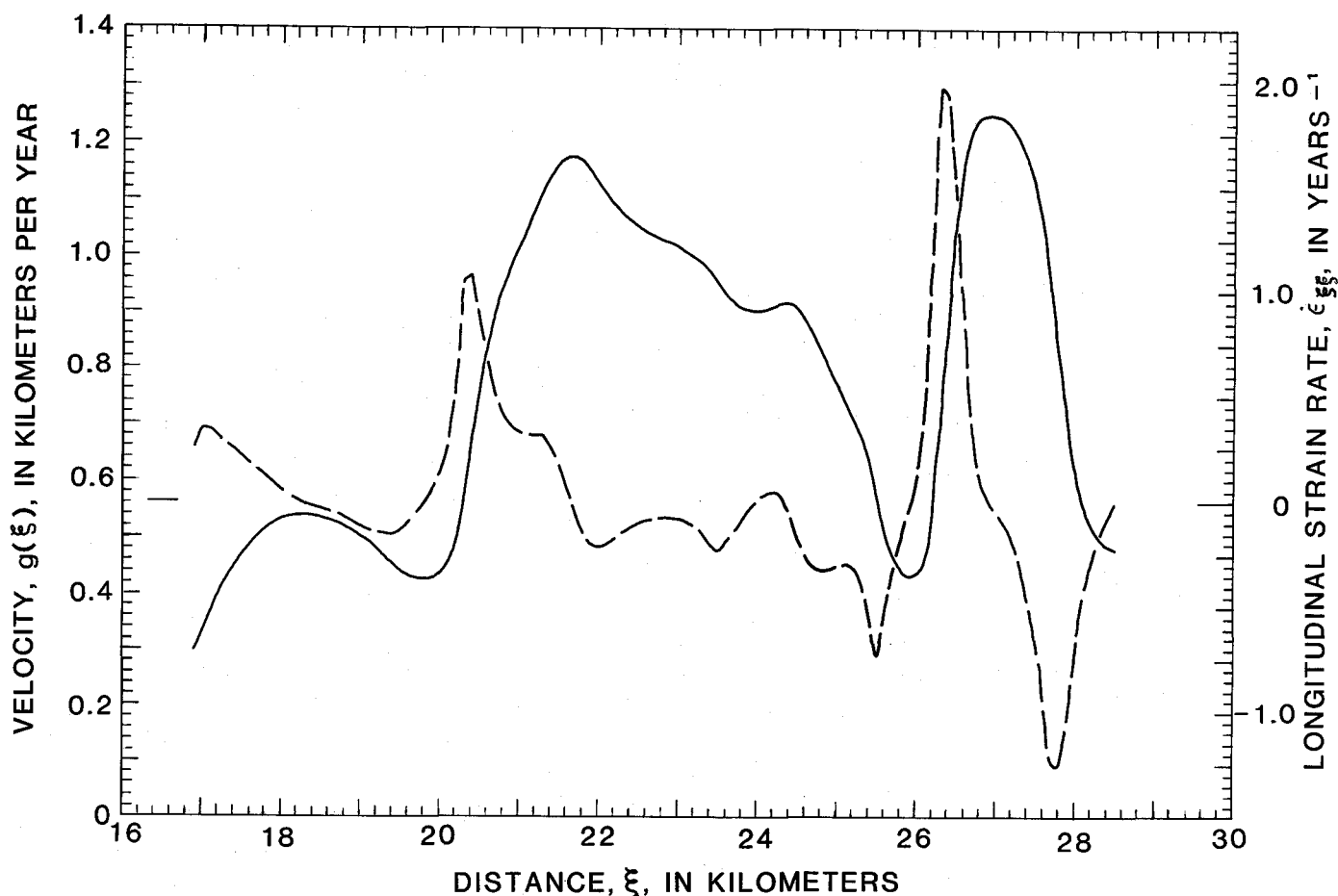
FIGURE 15.—Velocity function V\xi=g(\xi) obtained as reciprocal of curve in figure 14 (solid). Also shown is its longitudinal strain rate (dashed).
