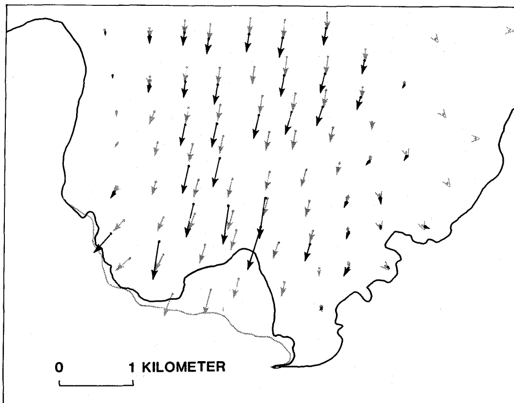
FIGURE 23.—Terminus configuration on June 2, 1977 (light), and on August 29, 1977 (heavy), combined with average velocity vectors for June 2 through July 7, 1977 (light), and for August 29 through November 8, 1977 (heavy), demonstrating acceleration and convergence induced in velocity field by embayments. Vector lengths represent 100-day displacements. Open arrows indicate flow direction where actual vectors are too small to show.
