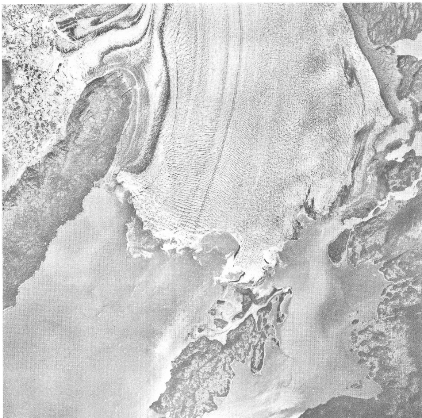
FIGURE 4.—Vertical aerial photograph from about 7,000 m above sea level showing terminus, including a large embayment toward the east edge, and the lowest 6 km of the lower reach, August 26, 1978. North is to the top.
