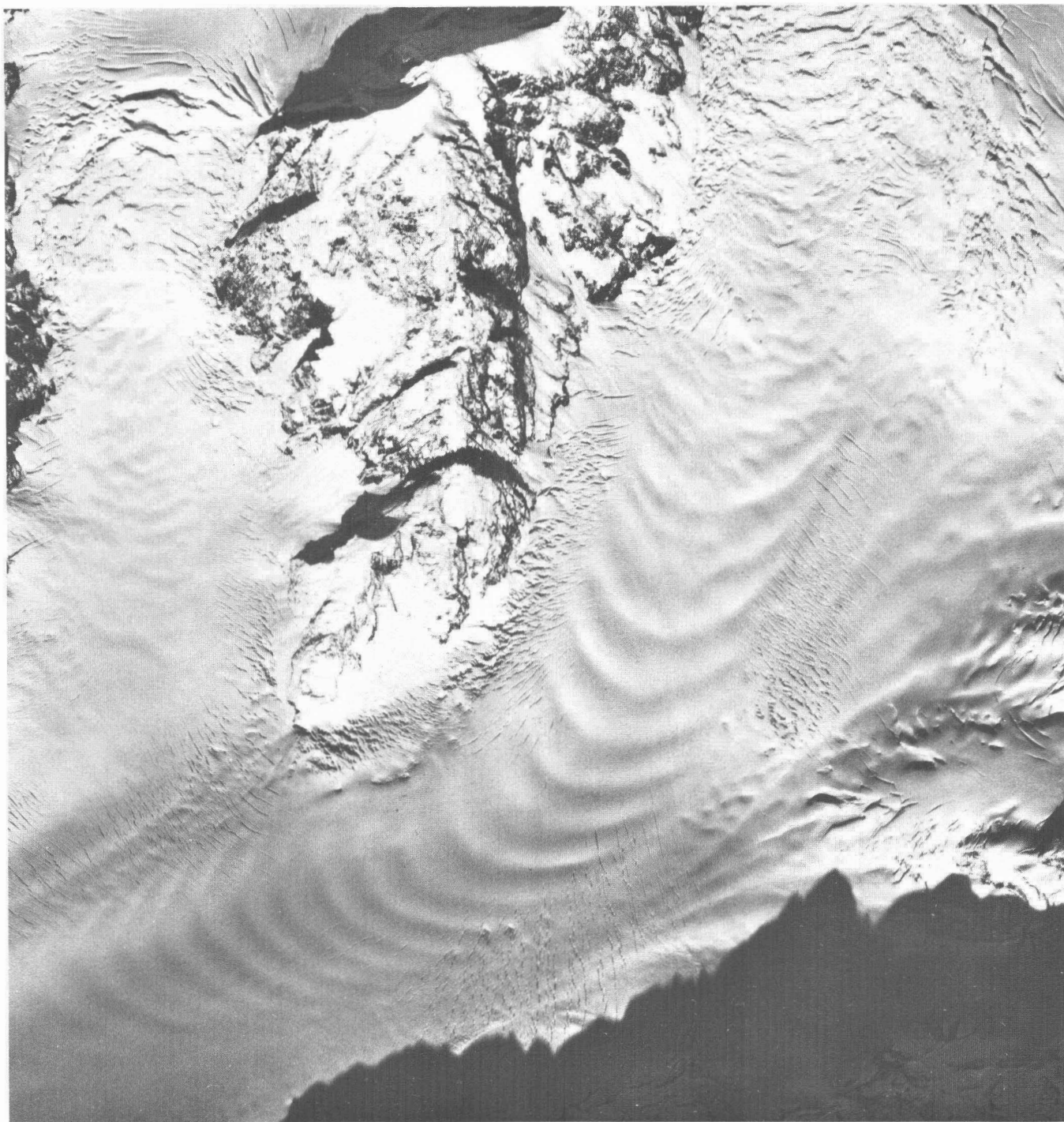
FIGURE 8.—Vertical aerial photograph from about 7,000 m above sea level showing wave ogives downglacier from an unnamed icefall upglacier from the west branch of Columbia Glacier, September 26, 1981.
