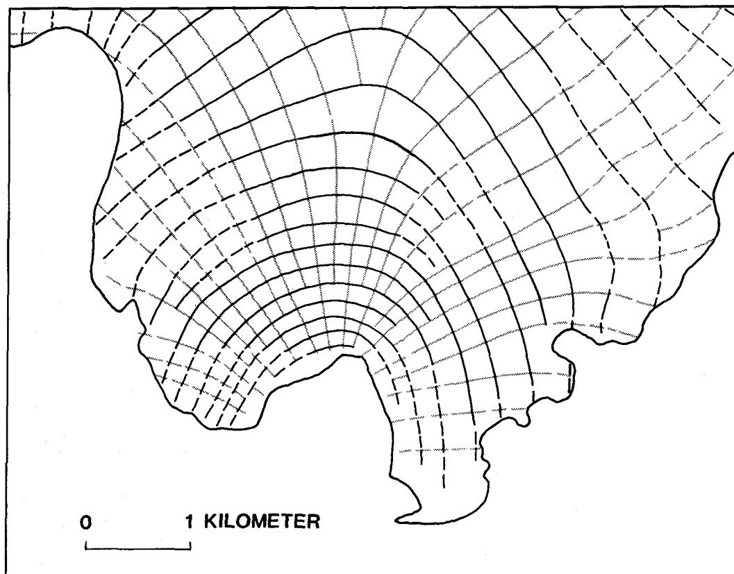
FIGURE 24.—Trajectories of principal axes of strain-rate tensor in vicinity of terminus, showing arch of compression around a large embayment. Strain rate determined from average velocity for August 29 through November 8, 1977; terminus configuration is that on August 29, 1977.
