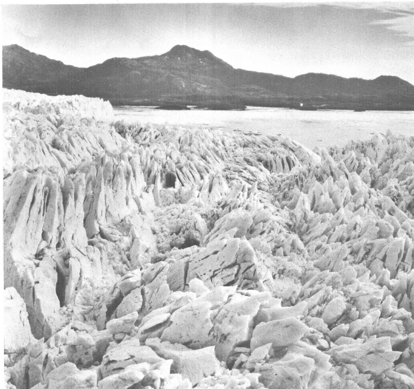
FIGURE 3.—Low-altitude oblique aerial photograph showing detail of the intensely fractured ice surface. This photograph shows an area about 1 km from the terminus and about 1 km from the west margin, view to south-southeast. Flow is diagonal to the right and away from the camera. U.S. Geological Survey photograph No. 75M5-62, by L. R. Mayo, October 8, 1975.
