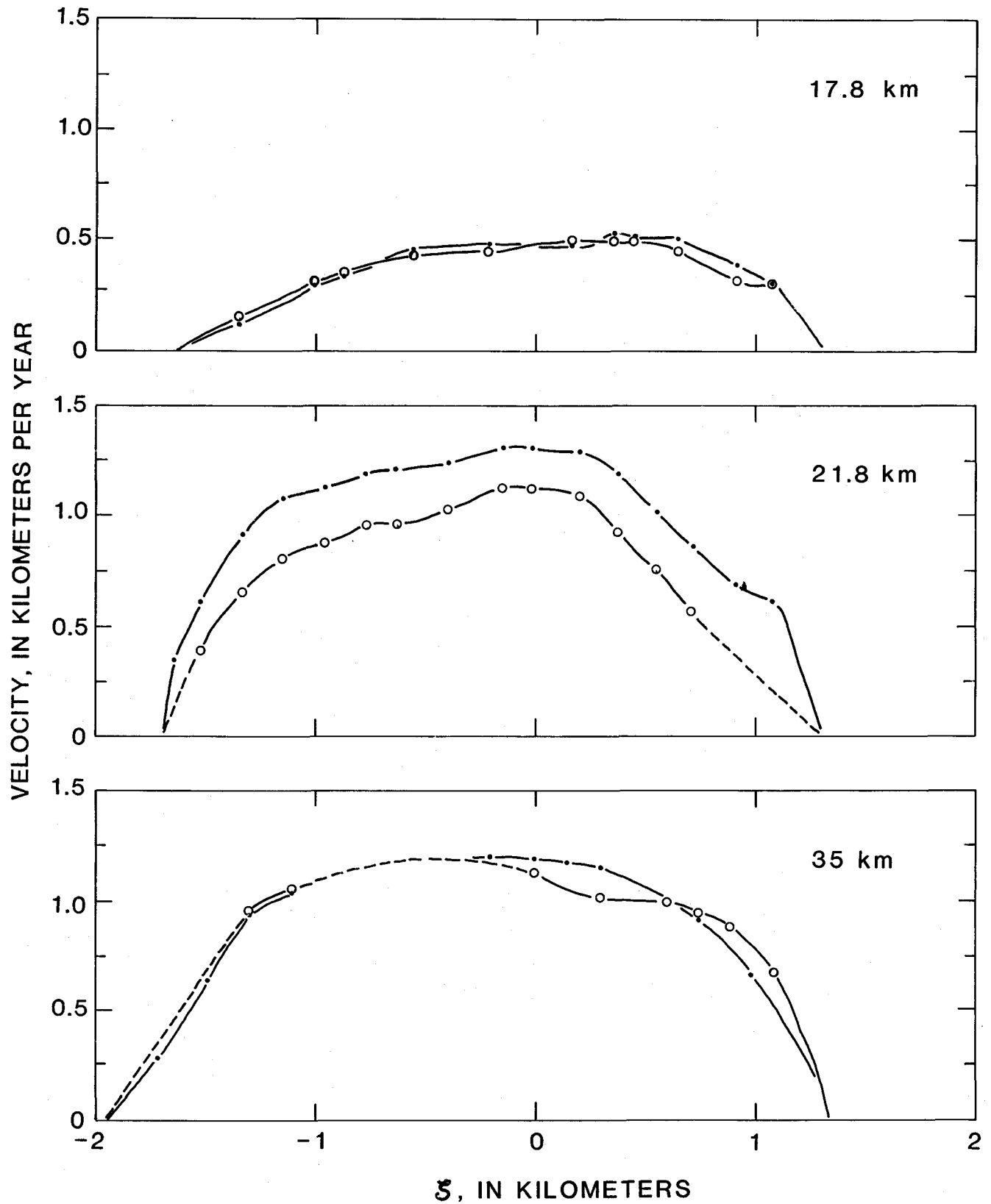
FIGURE 16.—Transverse velocity profiles for \xi=17.8 , \xi=21.8 , and \xi=35.0 km for April 19 to June 11, 1978 (circles), and for June 11 to July 30, 1978 (dots), illustrating data of table 5.
