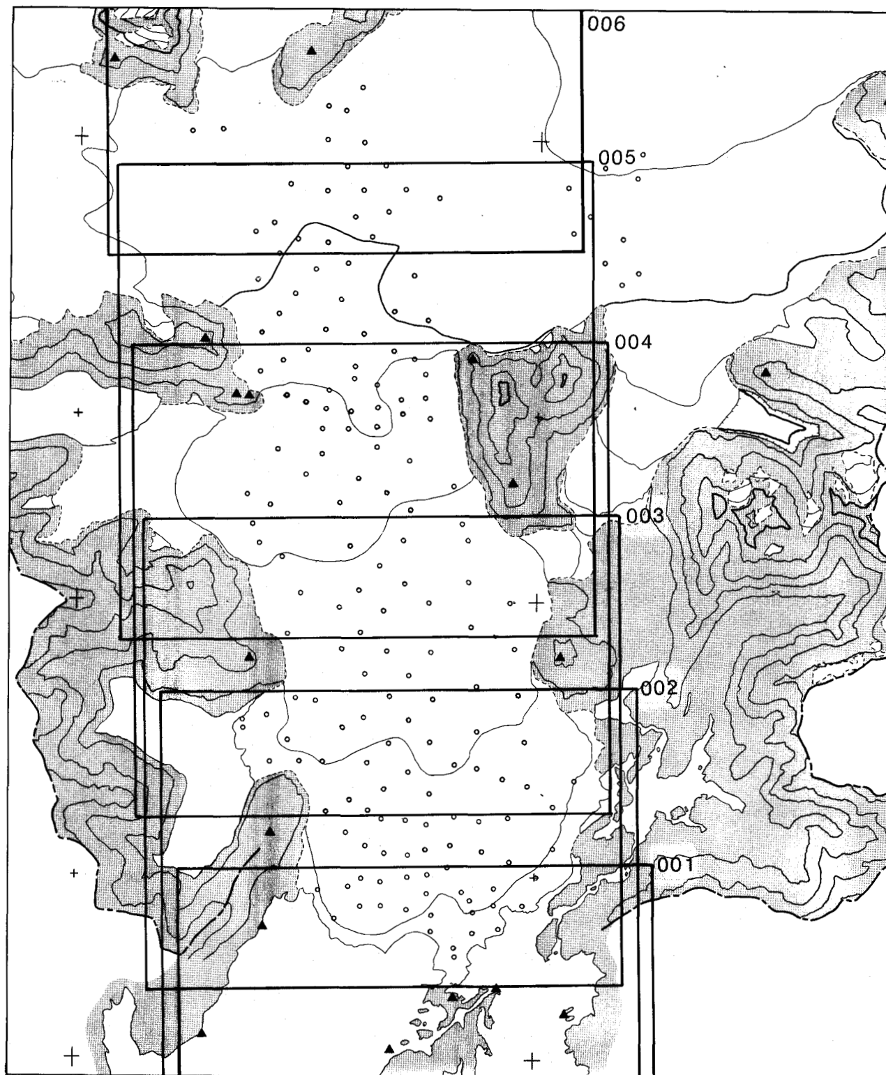
FIGURE 5.—Typical flight plan, showing coverage of each of six vertical aerial photographs. Open circles indicate a typical array of photogrammetrically determined glacier points. Triangles indicate survey stations, used for field control. Contour interval is 100 m.
