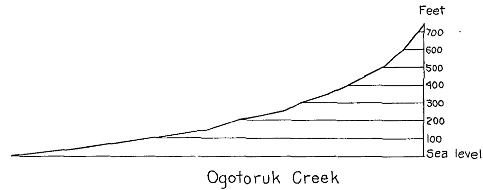
Plate 3.- Profiles of representative streams, vicinity of the Chariot site (After R. H. Campbell, U. S. Geological Survey)
